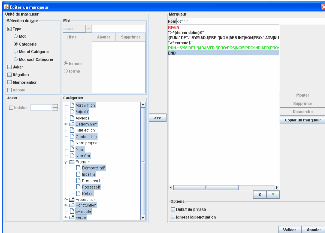
Figure 2. CAMÉLÉON Pattern Editor. The pattern presented here, called definir , mainly searches for forms like “X is defined as Y”. The user preferred not to specify where the defined concept could appear in a sentence ( BEGIN is in the X colour), but gave several constraints (list above END ) on how Y (the defining term) could be formulated.
