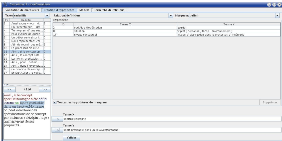
Figure 4. Text Fragment Extraction. Checking the definir pattern (for definition relations).
