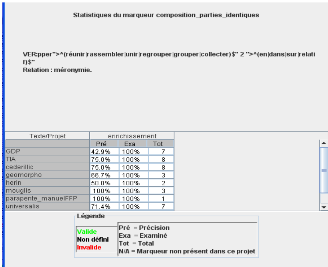
Figure 5. Example of statistical analysis of the pattern “composition_parties_identiques”. For each corpus it has been evaluated against (list in the left hand column) in a particular project (here, “enrichissement”), a measure of precision (Pré) is given, together with the percentage of analysed (Exa) sentence matches and with the absolute quantity of sentence matches (Tot).
