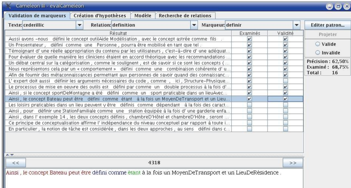
Figure 3. CAMÉLÉON Pattern Evaluation Screen. Given a text ( texte ), a relation type ( relation ) and a pattern, the user may ask to match the pattern to the text ( projeter ). Results are text excerpts (sentences) listed for checking. Selecting one of these sentences (the highlighted one) makes it possible to read the whole sentence that matches the pattern in the lower frame. Coloured words correspond to those identified as possible related concepts (X and Y). After validating or rejecting as many sentences as requested ( validate check boxes), the user may decide to modify the pattern ( Editer patron ), reject or validate it ( invalide or valide radio-button on the right). The precision score displayed on the right may guide this decision.
