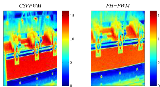
Fig. 15. Temperature increase in degrees Celsius measured for the converter for the CSVPWM technique and for the PH-PWM technique.
