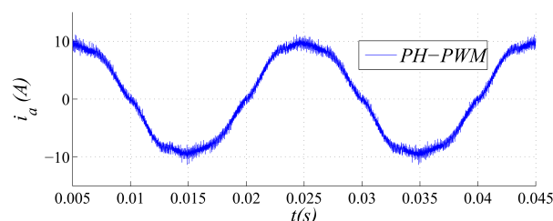
Fig. 16. Measured i_a for the considered working point and for the PH-PWM technique with \beta = 0.075 .
