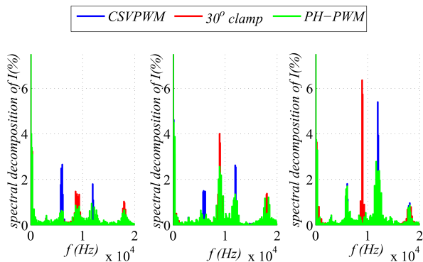
Fig. 13. Experimental spectral decomposition of the line current for the three PWM techniques for a DC bus voltage of 150V, 190V and 250V, respectively.
