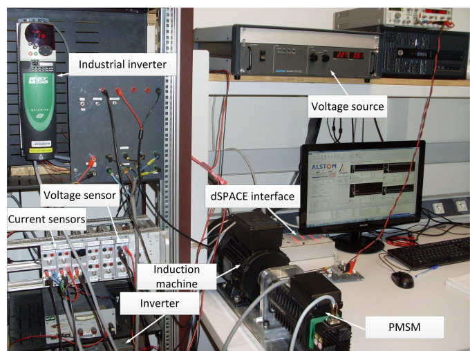
Fig. 8. Motor test-bench used for the experiment.
