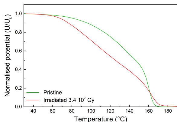
Figure 4: Normalised potential thermograms of pristine and irradiated samples
