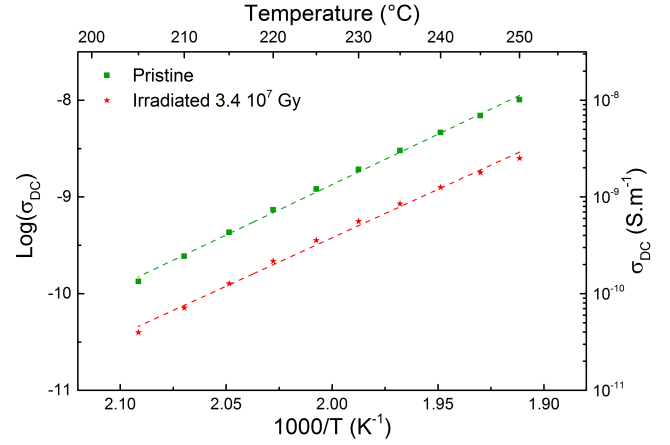
Figure 3: Arrhenius diagram of DC conductivity for the pristine and irradiated samples. Points represent experimental data while dashed lines represent fitted data
