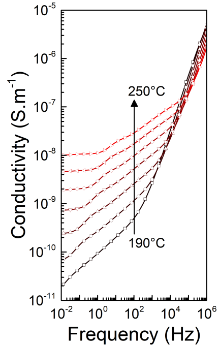
Figure 2: Frequency behaviour of the conductivity isotherms from 190 ^{\circ}\text{C} to 250 ^{\circ}\text{C} by 10 ^{\circ}\text{C} step for a pristine sample
