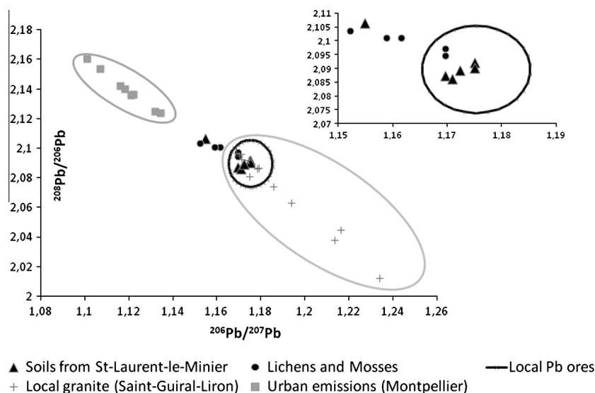
Fig. 3. Lead isotopic data for soil, lichen and moss (this study) and urban emission (Monna et al., 1997).
