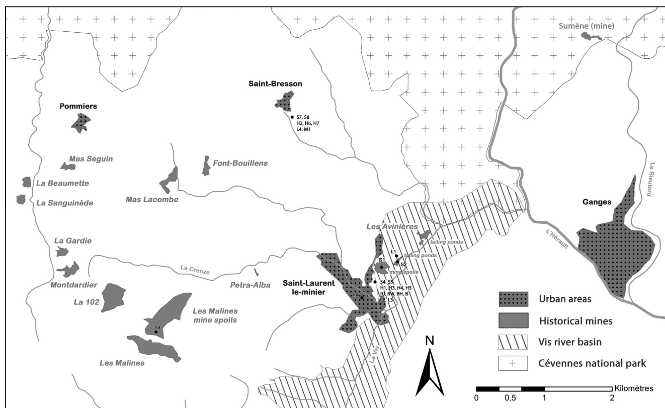
Fig. 2. Detailed map of the sampling area within the les Malines mining district.
