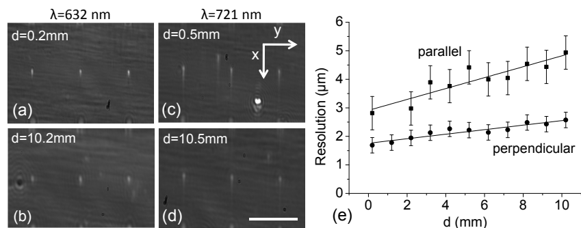
Fig. 4. Very-small-FOV SPR images of less than 1- \mu\text{m} -wide PDMS pillars in water at increasing distance d from the imaging side edge of the prism. SPW propagate downward. (a and b), at \lambda = 632 nm. (c and d), at \lambda = 721 nm. Images were taken with a gold-coated N-SF66 prism ( A_p = 83^\circ ) in the configuration of Fig. 1(b). (e) Resolution perpendicular and parallel (before the step) to the SPW with respect to the distance d at \lambda = 632 nm in water with a N-SF66 prism. Each point is an average of 1 to 3 PDMS pillars. The constant error bars are equal to the maximum difference observed for each orientation. Scale bar: 50 \mu\text{m} .
