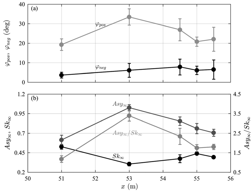
Figure 7. (a) Cross-shore variation of phase shifts \varphi_{pos} and \varphi_{neg} (maximum values in their near-bed profiles, as shown in Figure 6 for x = 53 m and x = 55 m) between x = 51 m and x = 55.5 m; (b) cross-shore evolution of Asy_{\infty} , Sk_{\infty} , and Asy_{\infty}/Sk_{\infty} between x = 51 m and x = 55.5 m. Values are averaged over all runs per location with associated error bars marking \pm 1 standard deviation.
