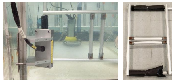
Figure 3: Ladder shaped target and Bathyswath V1 transducer
