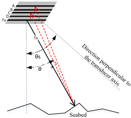
Figure 1 Basic setup of Interferometric Sonar System
