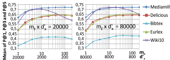
Figure 3. Evolution of the performances with respect to the number of tree at iso- (m_F \times d'_x) .
