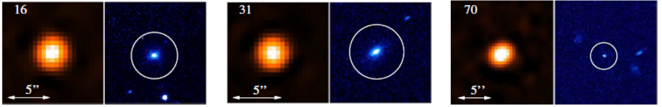
Fig. 2. Radio and optical images from Chiaberge et al. (2009) for the COSMOS-FRI sources in our sample. For each source, the image in the left panel is from the VLA-COSMOS survey ( Schinnerer et al. 2007 ), while in the right panel the HST-COSMOS ACS image (F814W) is shown ( Koekemoer et al. 2007 ).
