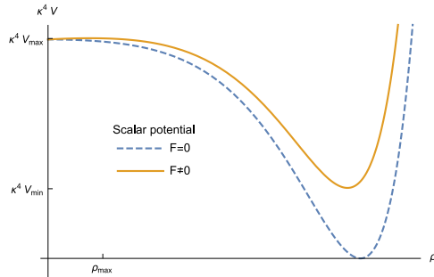
Fig. 2. This plot shows the scalar potentials in F = 0 and F \neq 0 cases. When F = 0 , we have a local maximum at \rho_{\max} = 0 and a global minimum with zero cosmological constant. For F \neq 0 , the local maximum is shifted by a small positive value to \rho_{\max} \neq 0 . The global minimum now has a positive cosmological constant.
