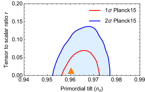
Fig. 3. A plot of the predictions for the scalar potential with F = 0 , b = 3/2 , A = 0.545 , B = 0.230 , \xi = -1.140 and q = 2.121 \times 10^{-5} in the n_s - r plane, versus Planck'15 results.
