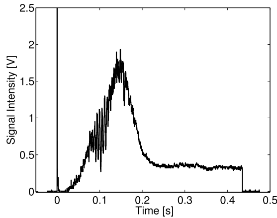
Figure 2. Raw signal showing the time evolution of the \gamma -ray flux over 450 ms.
