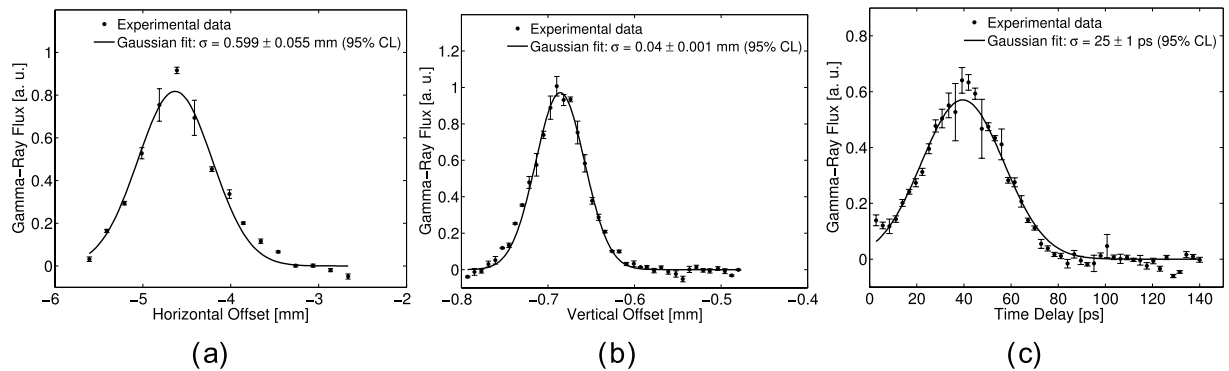
Figure 8. (a) Measured \gamma -ray flux as a function of the horizontal position of the Fabry-Perot cavity relative to the electron beam. (b) Measured \gamma -ray flux as a function of the vertical position of the Fabry-Perot cavity relative to the electron beam. (c) Measured \gamma -ray flux as a function of the phase shift between the reference clock of the accelerator and the laser oscillator responsible for the synchronization of the passage of the laser and electron beams at the interaction point. The error bars represent the standard error on the mean value.
