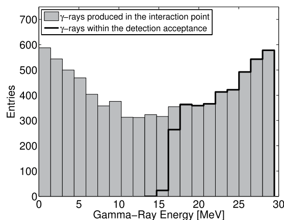
Figure 7. Computed energy spectrum of the \gamma -rays produced by Compton scattering of a 1034 nm laser beam off a 1.28 GeV electron beam. Only the \gamma -rays with energies above 15 MeV are detected resulting in the average energy of the measured \gamma -rays being 24 MeV.
