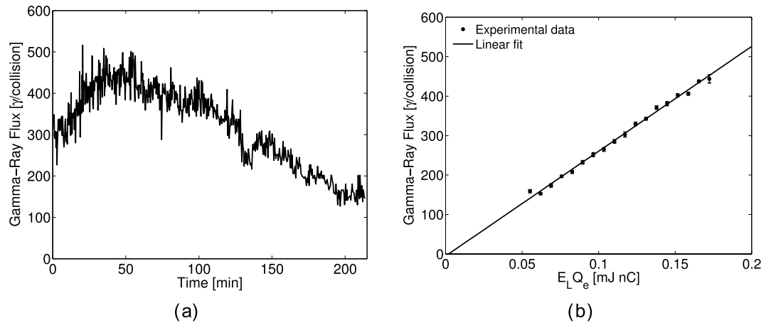
Figure 1. (a) Number of \gamma -rays produced versus time in the single-bunch operation mode. (b) Number of \gamma -rays produced per interaction as a function of the laser pulse energy E_L and the electron bunch charge Q_e product. The data points are fitted with a first order polynomial. The error bars represent the standard error on the mean value.
