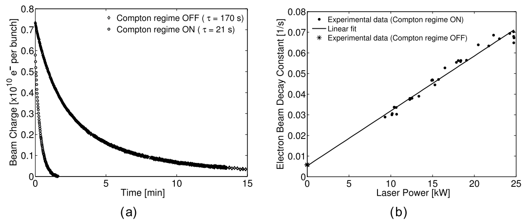
Figure 3. (a) Electron beam charge as a function of time in absence and presence of Compton scattering. A reduction by a factor 8 of the beam lifetime is observed due to the presence of Compton scattering. The laser power stored in the Fabry-Perot cavity during this measurement is 15 kW. (b) Decay constant as a function of the laser power stored in the Fabry-Perot cavity. The data points are fitted with a first order polynomial. The data points taken in absence of Compton scattering are excluded from the fitting procedure.
