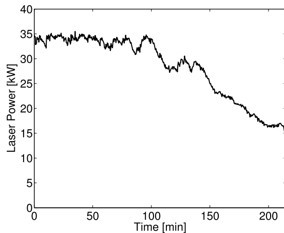
Figure 6. Laser power stored in the Fabry-Perot cavity measured during one of the data taking.
