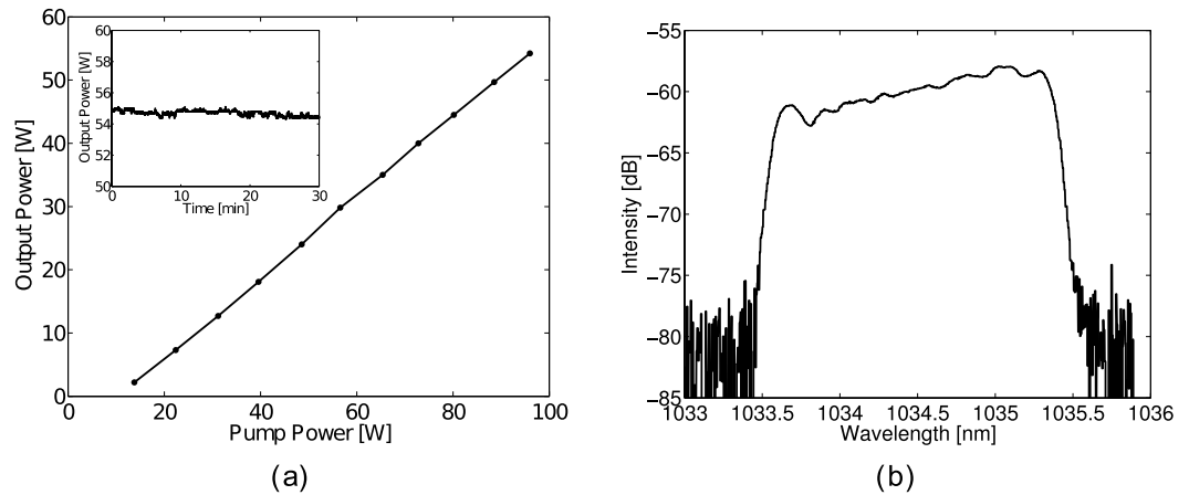
Figure 5. (a) Output power versus the pump power of the amplified laser beam. (b) Emission spectrum of the amplified laser beam. The square shape of the emission spectrum is due to the transmission bandwidth of the stretcher and compressor couple.
