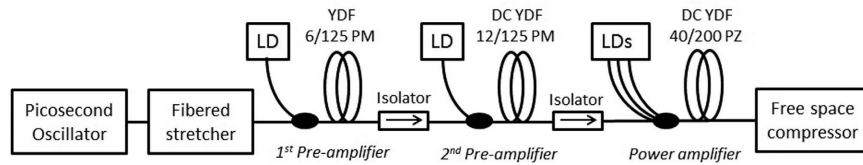
Figure 4. Schematic diagram of the high power picosecond pulsed laser, where LD and DC YDF denote a laser diode and a double clad Ytterbium doped fiber, respectively.
