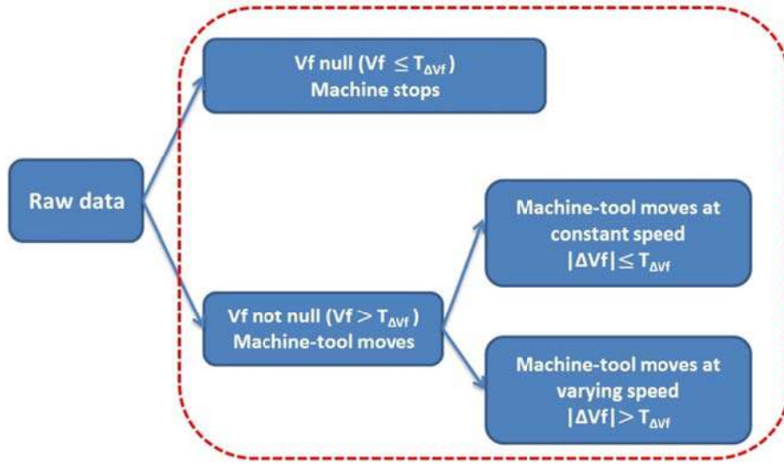
Fig. 2. Process of classification according the Feed rate Vf and \Delta Vf
