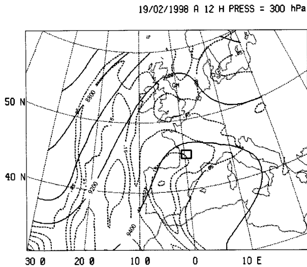
FIG. 1. The 300-hPa geopotential chart with humidity fields at 1200 UTC on 19 Feb 1998. The rectangular frame depicts the area of the cloud cirrus sampling discussed in this paper.
