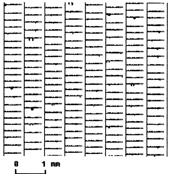
FIG. 8. Same as Fig. 4, except measurements performed between 1426:56 and 1527:03 near the cirrus cloud top (10 800 m MSL/ -60^{\circ}\text{C} ).
