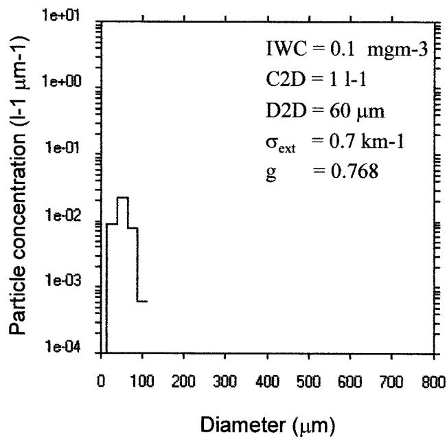
FIG. 8. Same as Fig. 4, except measurements performed between 1426:56 and 1527:03 near the cirrus cloud top (10 800 m MSL/ -60^{\circ}\text{C} ).
