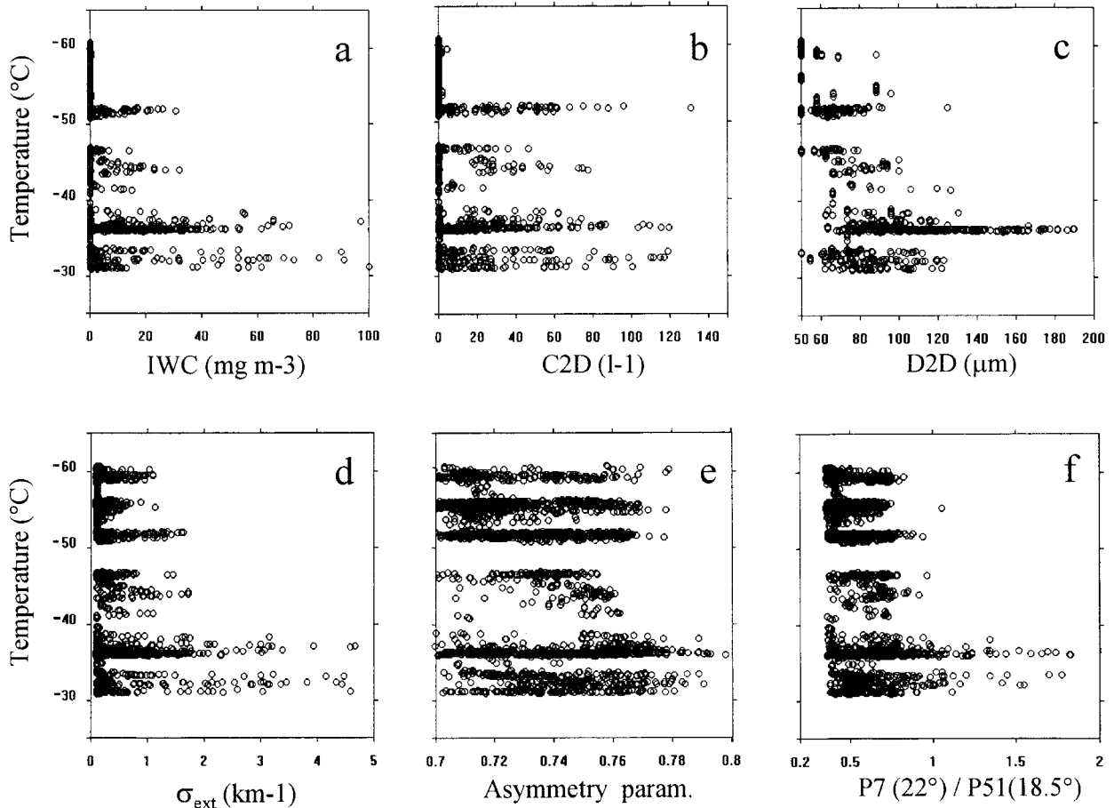
FIG. 7. Vertical profiles of cirrus uncinus microphysical and optical parameters: (a) IWC, (b) 2D-C ice particle concentration, (c) 2D-C mean diameter, (d) extinction coefficient, (e) asymmetry parameter, and (f) P7:P51 ratio.
