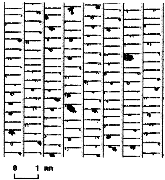
FIG. 6. Same as Fig. 4, except relative to cirrus sampled between 1537:09 and 1537:16 (7600 m MSL/ -35^{\circ}\text{C} ).
