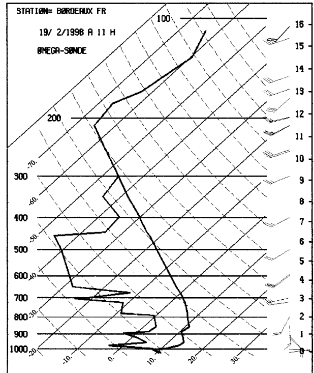
FIG. 2. Vertical sounding of the air, dewpoint temperatures, and wind obtained in Bordeaux, France, at 1100 UTC on 19 Feb 1998.
