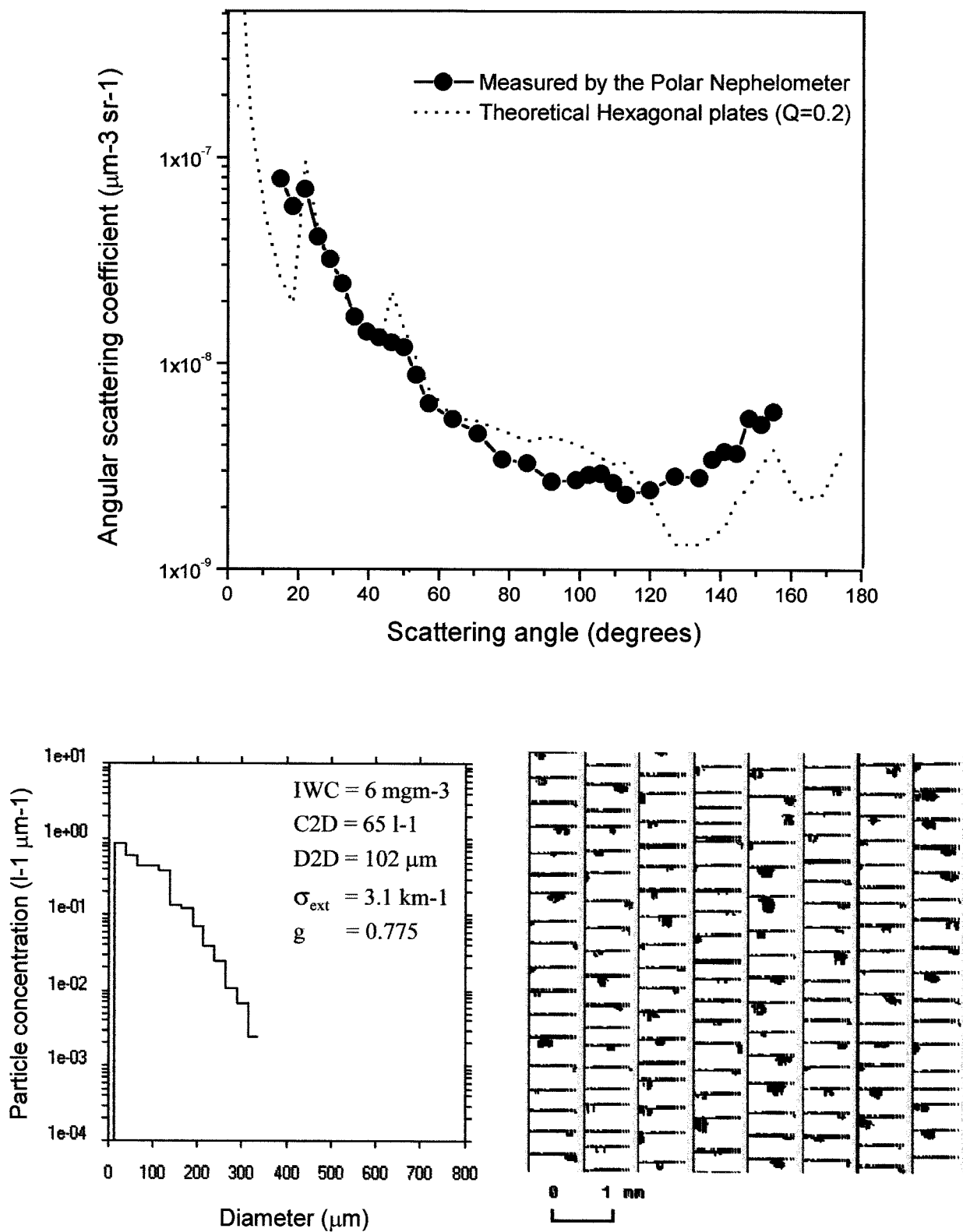
FIG. 5. Same as Fig. 4, except relative to cirrus sampled between 1532:52 and 1532:57 (7600 m MSL/ -35^{\circ}\text{C} ).
