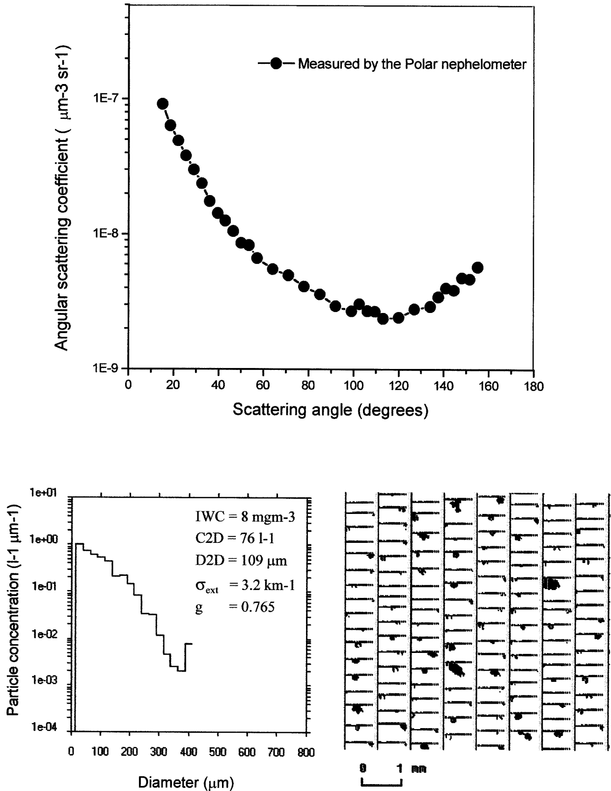
FIG. 6. Same as Fig. 4, except relative to cirrus sampled between 1537:09 and 1537:16 (7600 m MSL/ -35^\circ\text{C} ).
