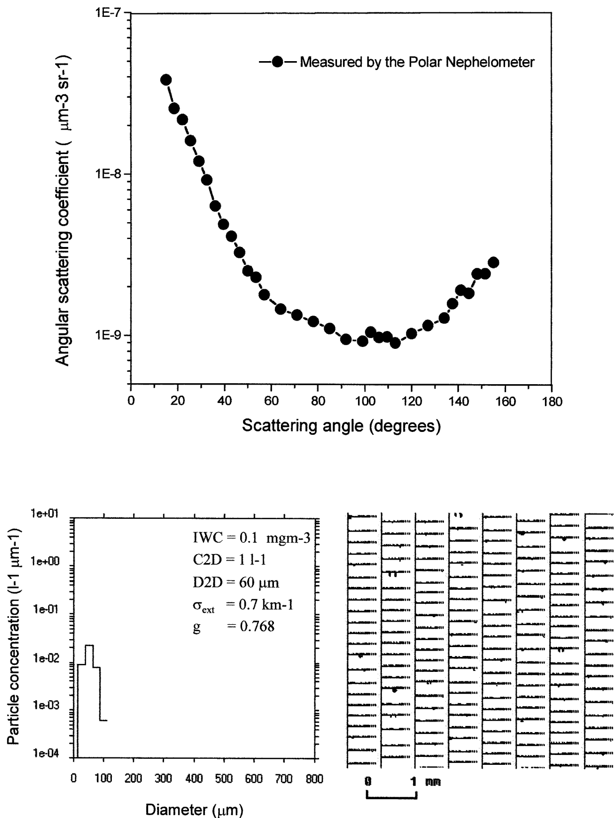
FIG. 8. Same as Fig. 4, except measurements performed between 1426:56 and 1527:03 near the cirrus cloud top (10 800 m MSL/ -60^\circ\text{C} ).
