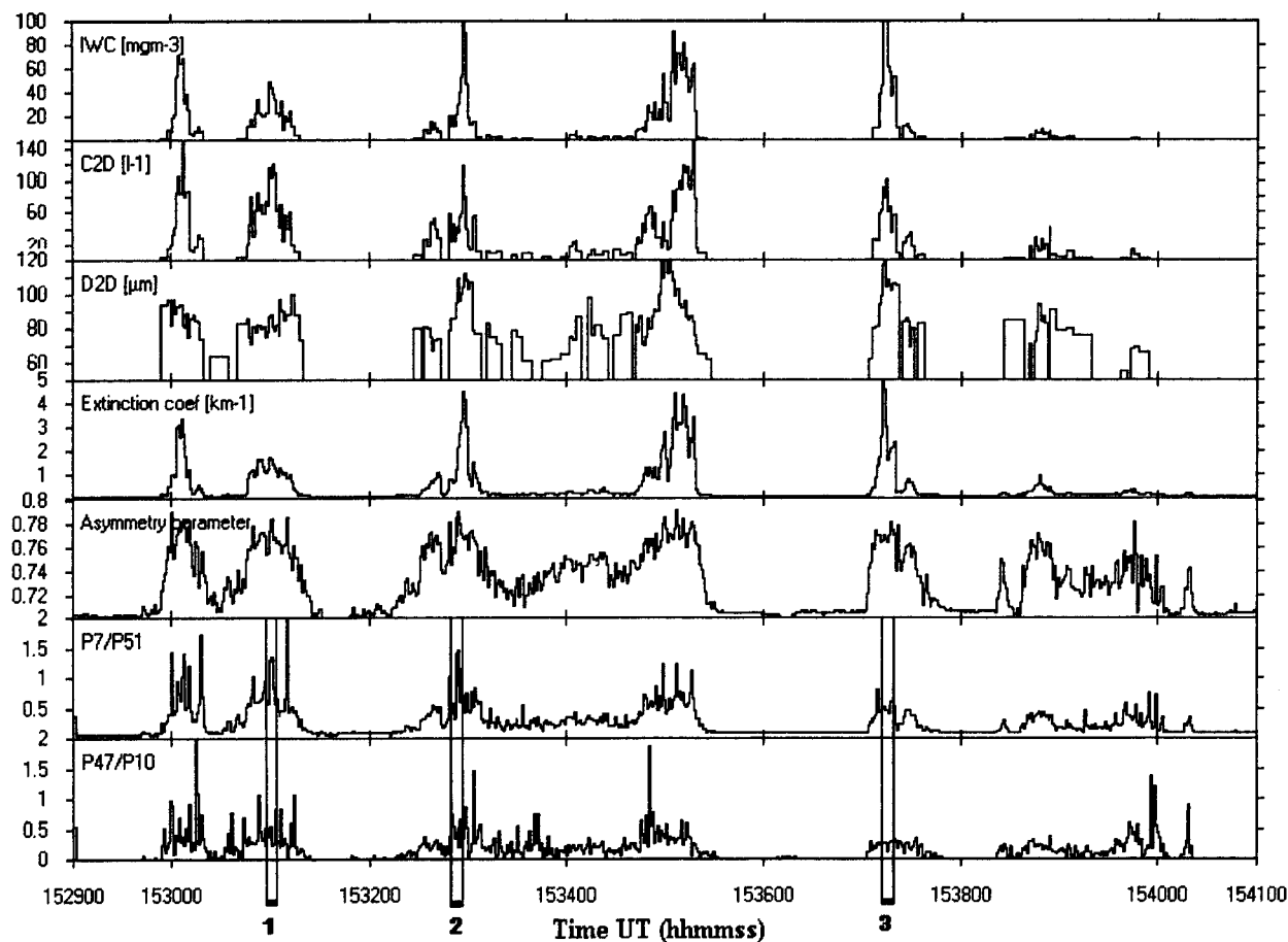
FIG. 3. Time series of the TBM700 parameters measured during the flight on 19 Feb 1998 at the 7600 m/ -35^{\circ}\text{C} level in cirrus uncinus clouds.
