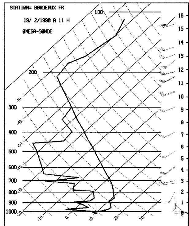
FIG. 2. Vertical sounding of the air, dewpoint temperatures, and wind obtained in Bordeaux, France, at 1100 UTC on 19 Feb 1998.
