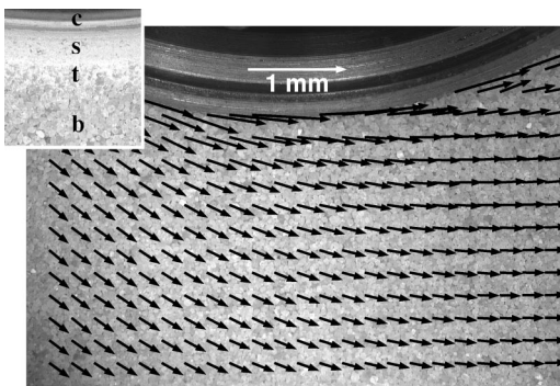
FIG. 2. Background is a raw digital picture taken through the observation window. It corresponds to an imposed slip \delta = 2.5 mm. Superimposed vectors represent the incremental displacement field \mathbf{du} in the sample. It is computed by applying CIV between this photo and the following one (taken in a 10-s delay). Subregions for correlation computation size 64 \times 64 px. The white arrow gives the scale of the plot. A detail of the shear band that develops after localization is included in the upper left corner of the image: c , rotating cylinder; s , shear band; t , transition layer; b , bulk, where original particles can be observed.
