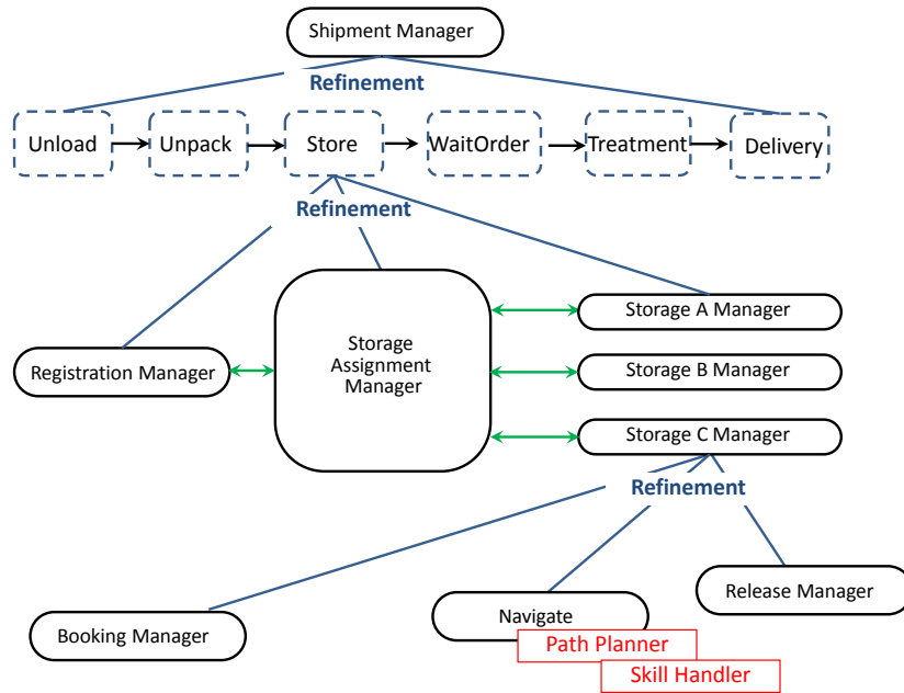
Figure 1: Deliberation components for a Harbor Organization Management facility.
