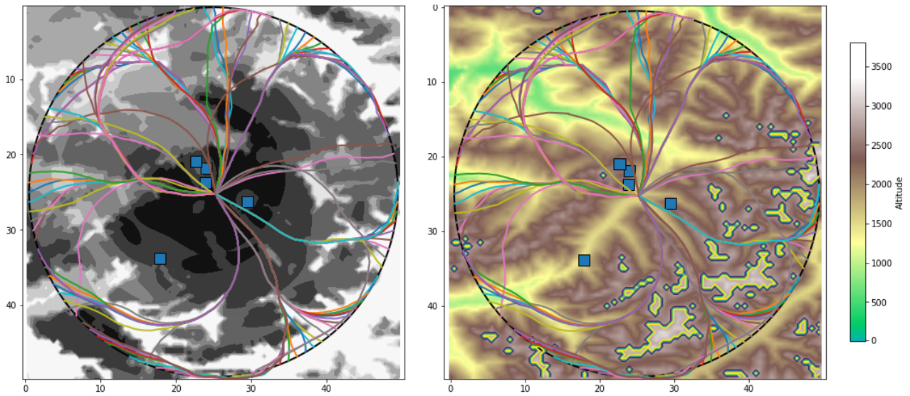
Figure 2: Threatening trajectories, from a circular region towards its center point, with optimized radar positions. (left) Positional factor \alpha_{\xi}(\mathbf{x}) in the cost map, where \xi is the radar configuration. (right) Digital elevation map.
