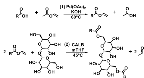
Scheme 1: Two-step procedure for the synthesis of trehalose diesters, (1) transvinylation step, (2) enzymatic esterification
