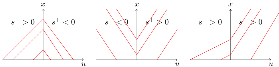
FIGURE 1. Solutions of (5) depending on the signs of s^- and s_+ : from left to right, solutions of (5a), (5b) and (5c)
