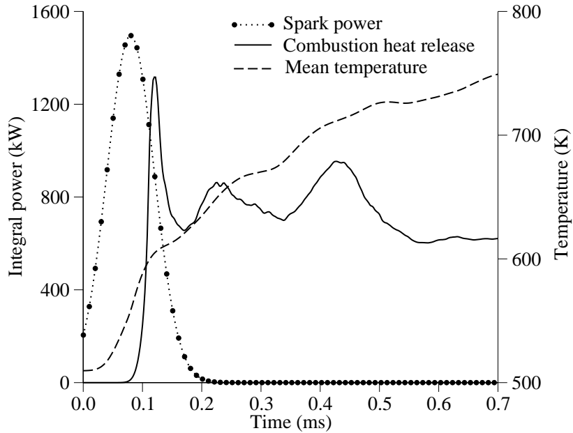
Figure 28: Total (spatially integrated) source term \dot{\omega}_{spark} , total heat release \dot{\omega}_T , and spatially averaged temperature.
