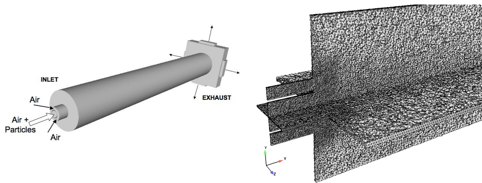
Figure 5: Computational domain and mesh of the Sommerfeld configuration.
