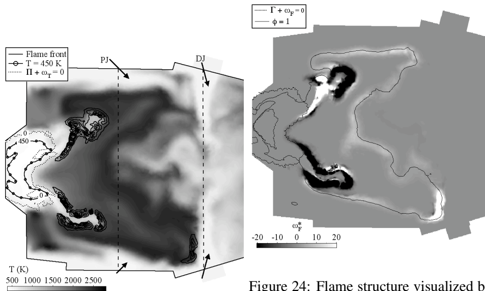
Figure 23: Flame front
