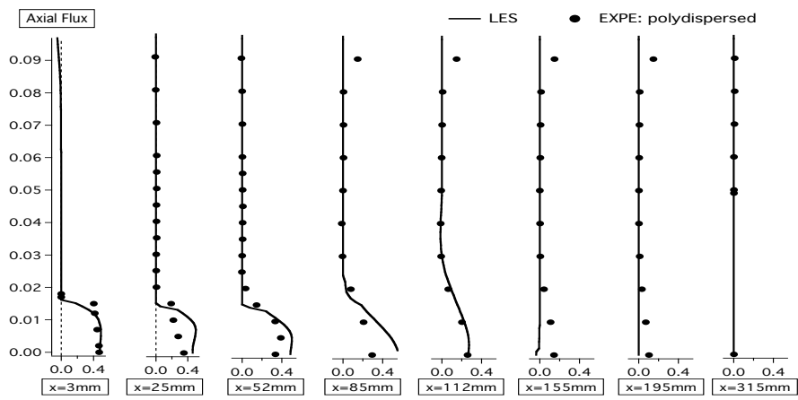
Figure 15: Axial liquid mass flux. Numerical simulations use 45 \mu m monodisperse droplets.
