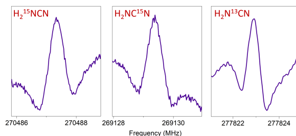
Fig. 2. Sections of the rotational spectrum of cyanamide displaying the J_{K_a, K_c} = 14_{1,14}\text{--}13_{1,13} transitions of three isotopic species within the 0^- tunneling state.
