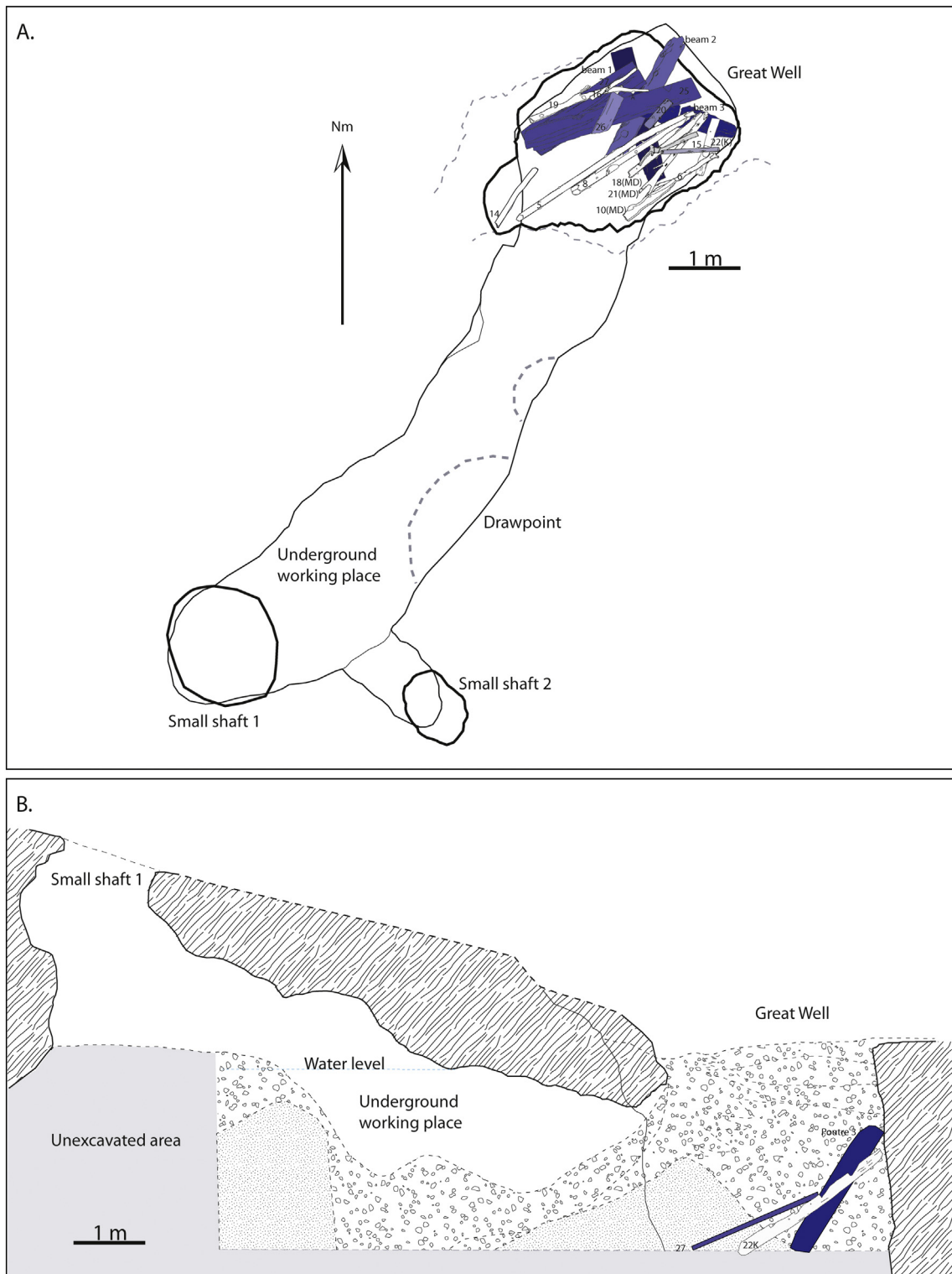
Fig. 4. A. Map view of the main Great Well woods (Bruno Ancel, Vanessa Py-Saragaglia). B. Cross-sectional view of the Great Well with only the main woods represented. All woods were accumulated on the large beams following the same inclination (Bruno Ancel, Vanessa Py-Saragaglia).
