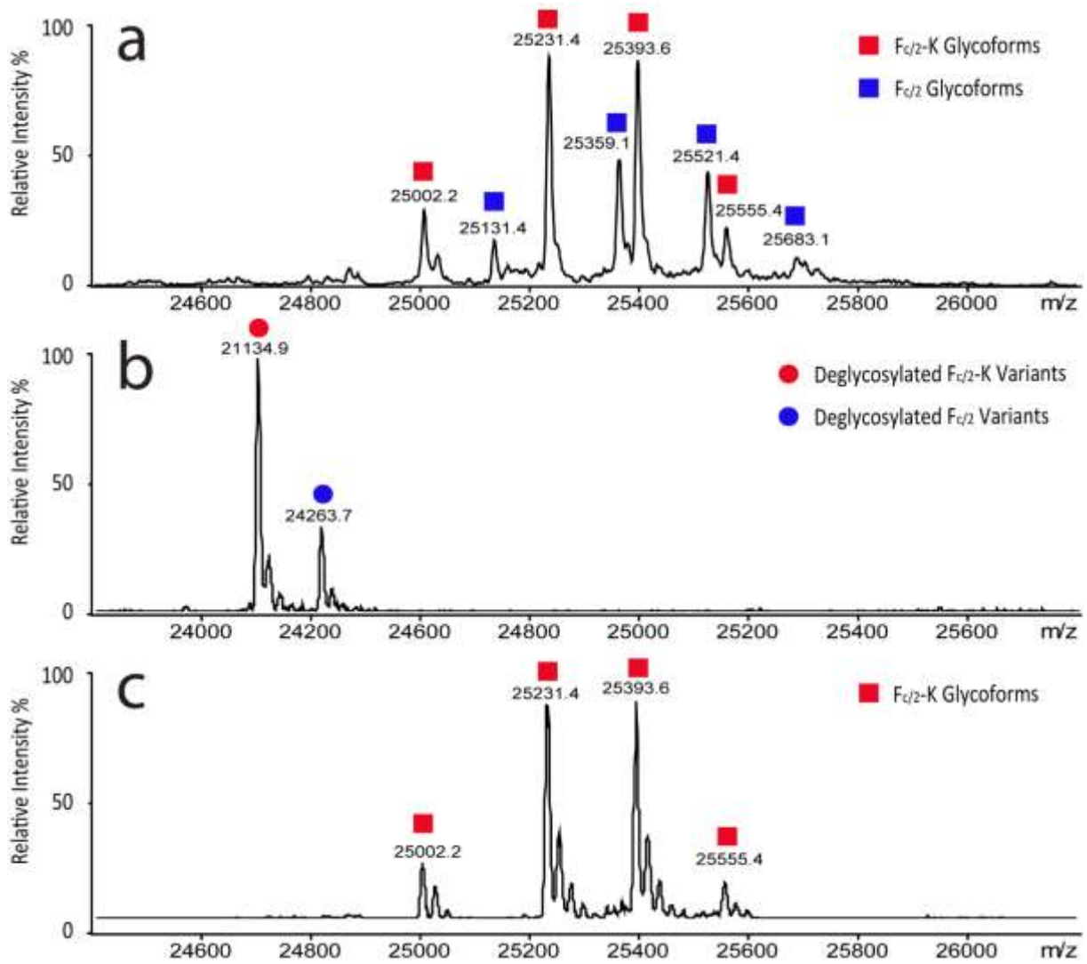
Fig. 4. F c/2 variants deconvoluted mass spectra of (a) IdeS digest cetuximab, (b) IgGZERO+IdeS digest cetuximab and (c) CP-B+IdeS digest cetuximab. Experimental conditions: 50%/49%/1%, acetonitrile/water/formic acid (v/v/v); sample concentration 1 μM.
