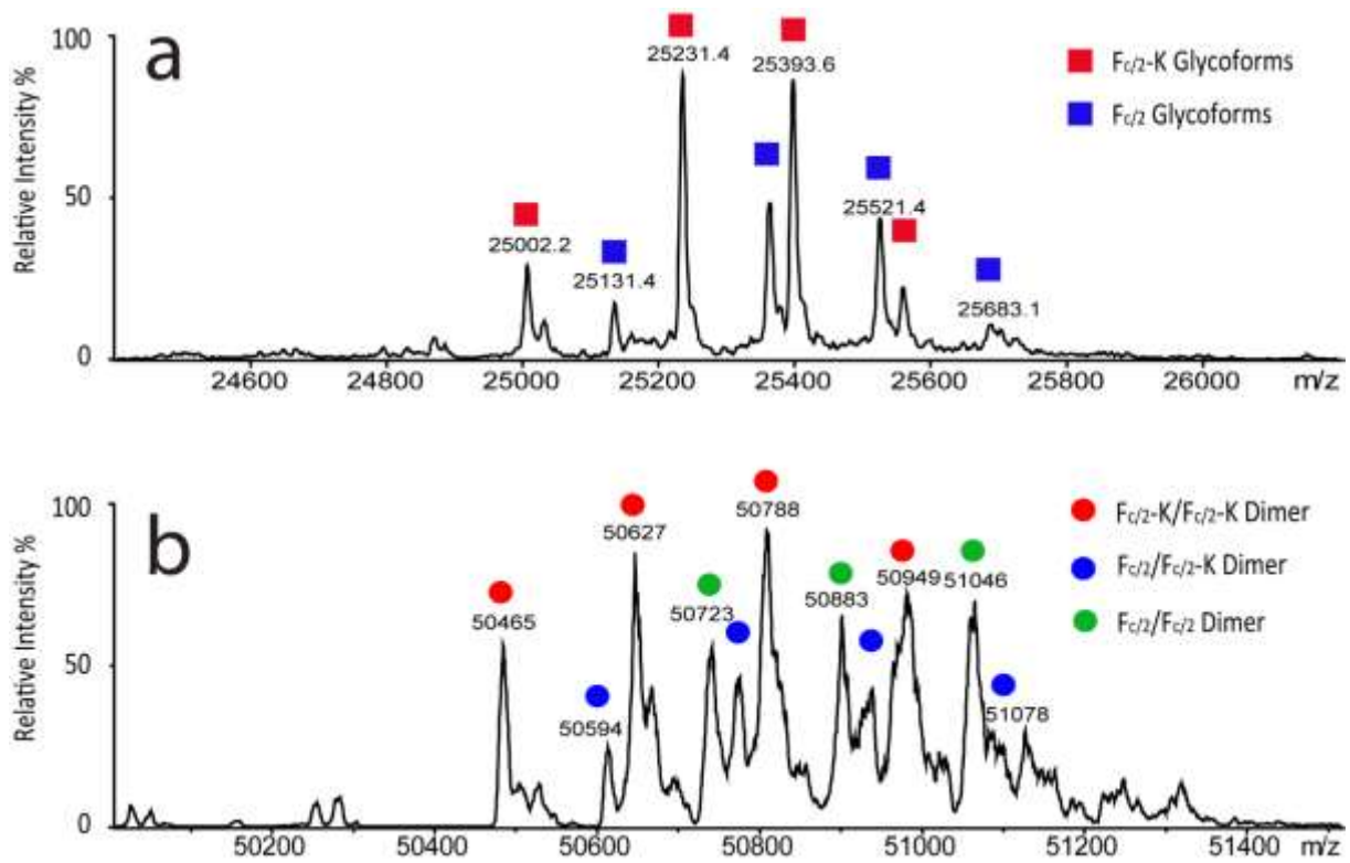
Fig. 5. Cetuximab F_{c1/2} variants deconvoluted mass spectra in (a) denaturing and (b) CZE conditions. Experimental conditions: denaturing conditions, 50%/49%/1%, acetonitrile/water/formic acid (v/v/v); CZE conditions, ammonium acetate 25mM, pH 5.7; sample concentration 1 \mu M.
