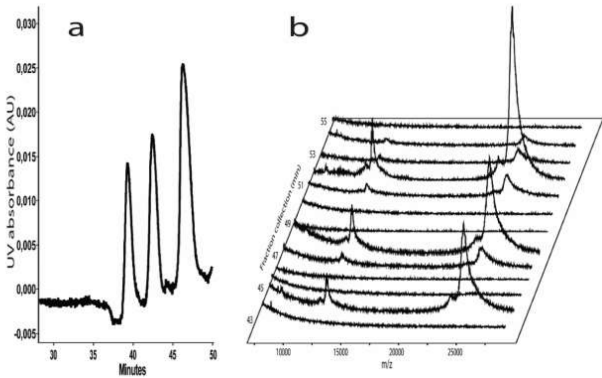
Fig. 2. CZE-UV off-line coupled to MALDI-MS via fractionation for a middle-up characterization of Cetuximab F c/2 variants. (a) CZE-UV electropherogram. (b) Analysis of CZE-UV fractions by MALDI-MS. CE Experimental conditions: See Fig. 1; MS condition: See Experimental section; sample, IdeS digest of cetuximab (5 µg/µL)
