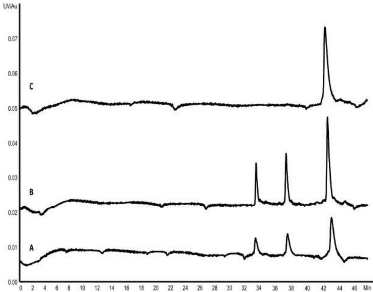
Fig. 3. Impact of glycosylation and lysine truncation on electrophoretic resolution. Electrophoretic separation of (A) cetuximab with IdeS treatment, (B) cetuximab with IgGZERO+IdeS treatment and (C) cetuximab with CP-B+IdeS treatment. Inlet BGE composed by a mixture of EACA 200 mM and ammonium acetate 25 mM pH 5.70 and outlet BGE by ammonium acetate 25 mM at pH 5.70.
