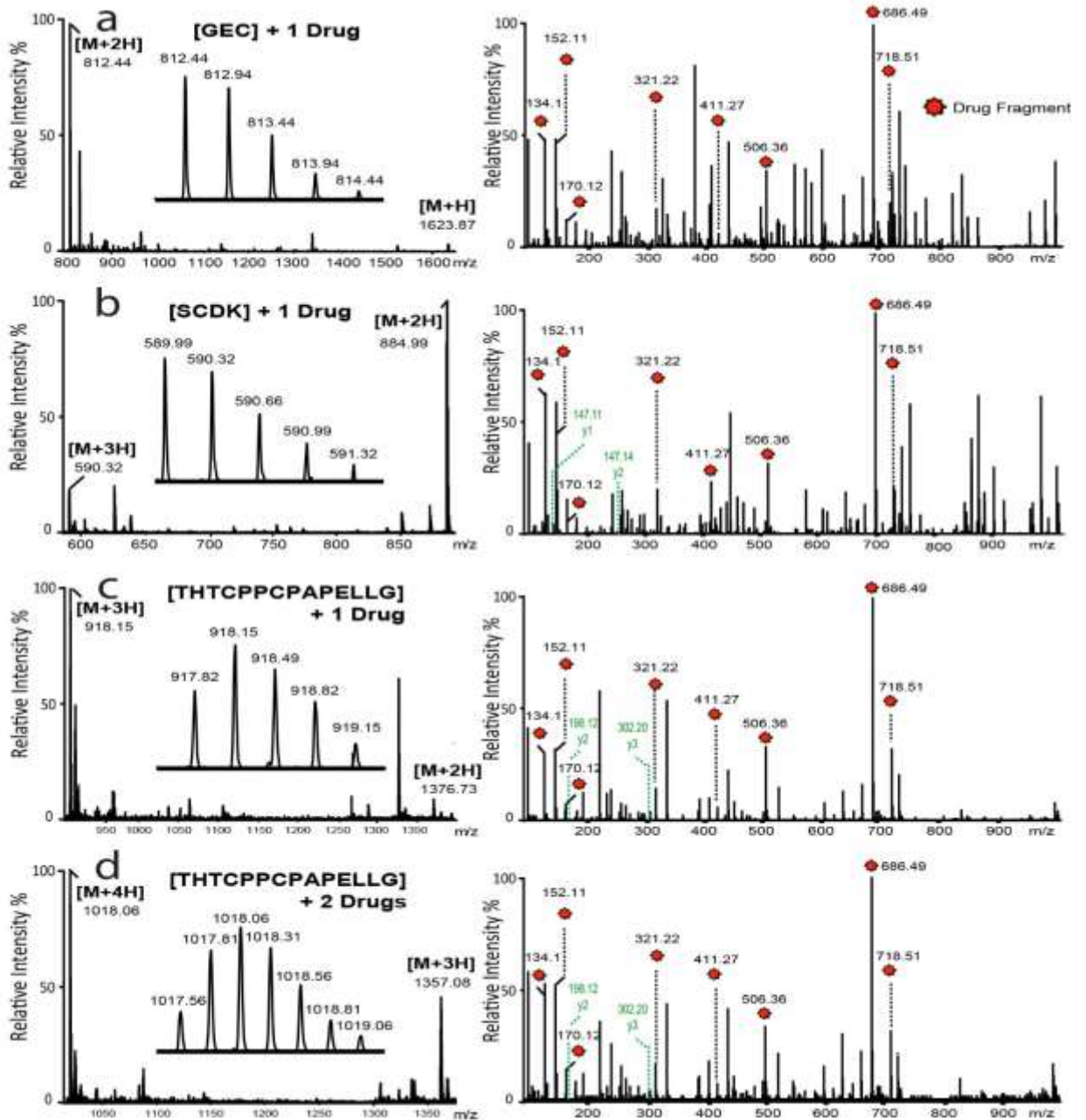
Figure 4. MS and MS/MS spectra of drug-loaded peptides. (a) [GEC] + 1 payload, (b) [SCDK] + 1 payload, (c) [THTCPPCAPELLG] + 1 payload and (d) [THTCPPCAPELLG] + 2 payloads
