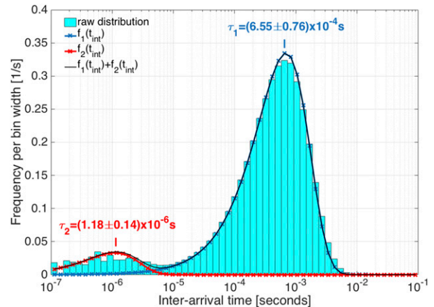
FIG. 11-11. Normalized frequency distribution of interarrival times recorded by a 2DS probe installed on a French Falcon aircraft during the collaborative 2014 HAIC/HIWC project on 18 Feb 2014. Solid lines represent best fits to modes of peaks describing naturally occurring particles and shattered artifacts, generated following approach of Jackson et al. (2014).
