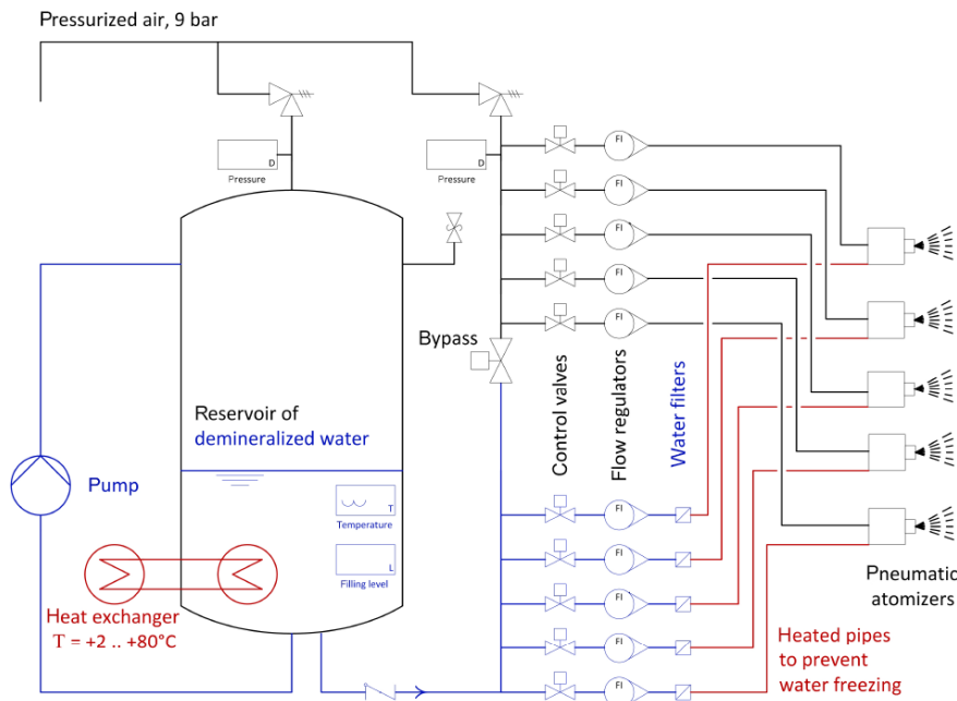
Figure 6. Spray system for low MVD and low LWC, and its supply system.
