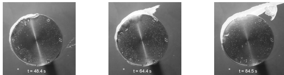
Figure 32. Side view of ice accretion when heating the cylinder, T_\infty = -5 \text{ }^\circ\text{C} , TWC = 6.8 \text{ g m}^{-3} and m_r = 0.5 .
