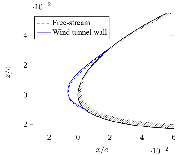
Figure 11. Inviscid wall effect on ice accretion for a AH-94-W-145 airfoil, c = 0.75 m, U_\infty = 40 m s -1 , T_\infty = -10 °C, LWC = 0.3 g m -3 , MVD = 15 μm and IWC = 0.
