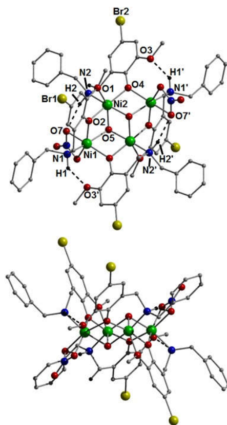
Figure 9 Crystal structure of one of the two [Ni(II)_4(\mu_3-OH)_2(L_6)_4](NO_3)_2 units observed in the a.s.u. of 8 as viewed perpendicular (top) and parallel (bottom) to the \{Ni_4\} plane. Majority of H-bonds have been omitted for clarity. Dashed lines represent intramolecular H-bonds at distances ( \text{\AA} ): N1(H1) \cdots O3' = 2.192 and N2(H2) \cdots O7' = 2.229 .
