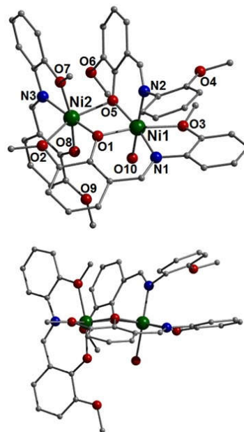
Figure 2 Crystal structure of [Ni(II)_2(L_3)_3(H_2O)](NO_3) \cdot 3MeOH \cdot 2H_2O ( 3 ) as viewed off-set and parallel to the Ni-O_{phen}-Ni plane. Hydrogen atoms have been omitted for clarity.
