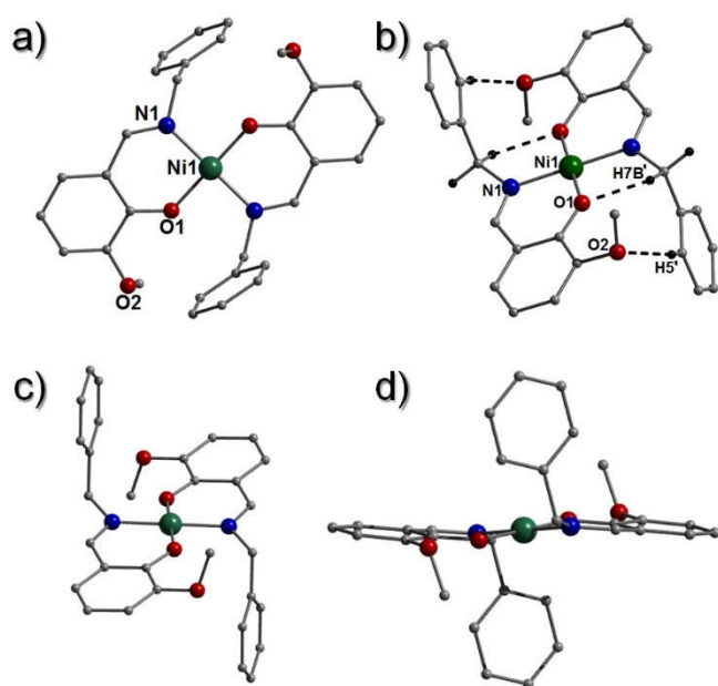
Figure 3 Crystal structure of [Ni(II)(L_4)_2] ( 4 ) as viewed perpendicular (a – c) and parallel (d) to the equatorial plane. Colour code: Ni (green), O (red), N (blue), C (grey). Majority of hydrogen atoms have been omitted for clarity. Dashed lines are intramolecular H-bonds at distances: O1 \cdots H7B'(C7') = 2.19 \text{ \AA} and O2 \cdots H5'(C5') = 2.34 \text{ \AA} . The additional ' symbol in the atom labels indicates that these atoms are at equivalent positions (1-x, 1-y, 1-z).
