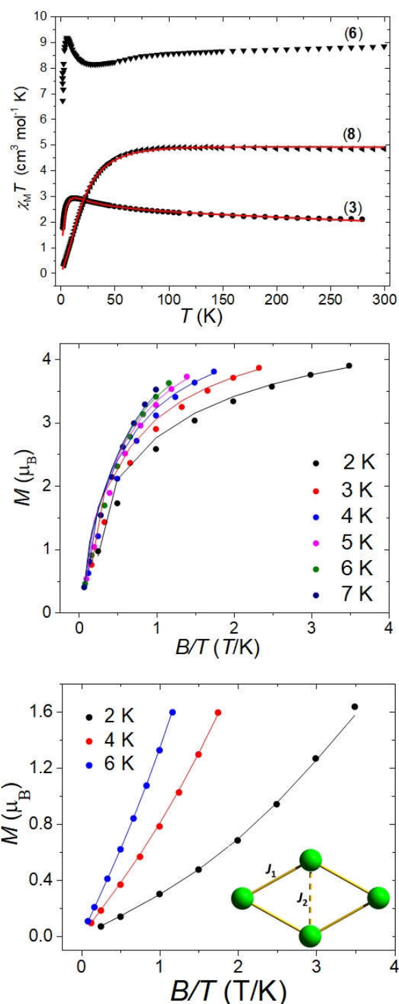
Figure 10 Top: Plot of \chi_M T versus T for complexes (3), (6) and (8). Middle: Reduced magnetisation data for complex (3). Bottom: Reduced magnetisation data for complex (8). The inset shows the exchange coupling scheme used to fit the data; \hat{H} = -2J_1(\hat{S}_1 \cdot \hat{S}_2 + \hat{S}_2 \cdot \hat{S}_3 + \hat{S}_3 \cdot \hat{S}_4 + \hat{S}_4 \cdot \hat{S}_1) - 2J_2(\hat{S}_2 \cdot \hat{S}_4) . The solid lines represent a simultaneous best-fit of the experimental susceptibility and magnetisation data as described in the main text.
