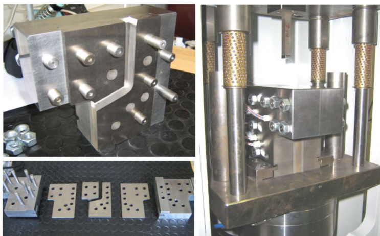
Figure 34. ECAP tool used for SPD treatments to Mg alloys, as developed by POINSARD Design and Tool SAS (Besançon, France). Up and left: the open channeling die, down-left: tools forming different angle channels, \Phi_E = 95^\circ, 105^\circ, 115^\circ, 125^\circ, and 135^\circ , right: ECAP system (die, punch) [36].
