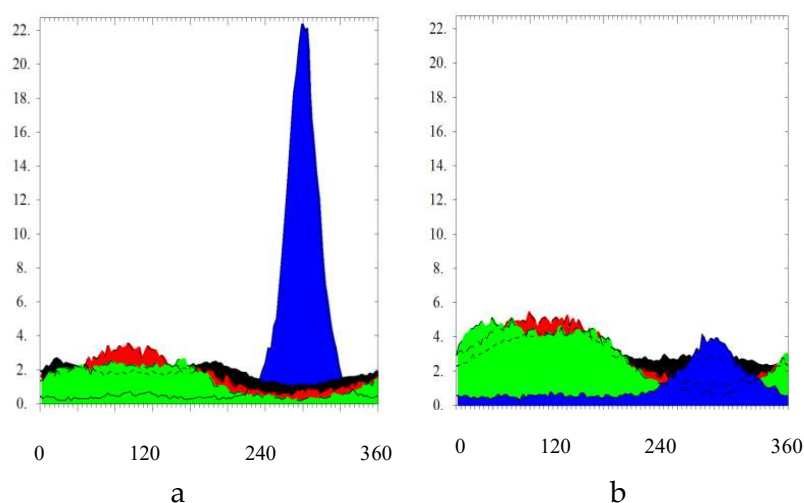
Figure 19. Texture integrated and normalized intensities of the four main crystallographic planes. (a)—after 1 pass (~A), (b)—after 9 passes B C . Colors are for: blue (002), red (100), black (101), and green (110) lines.
