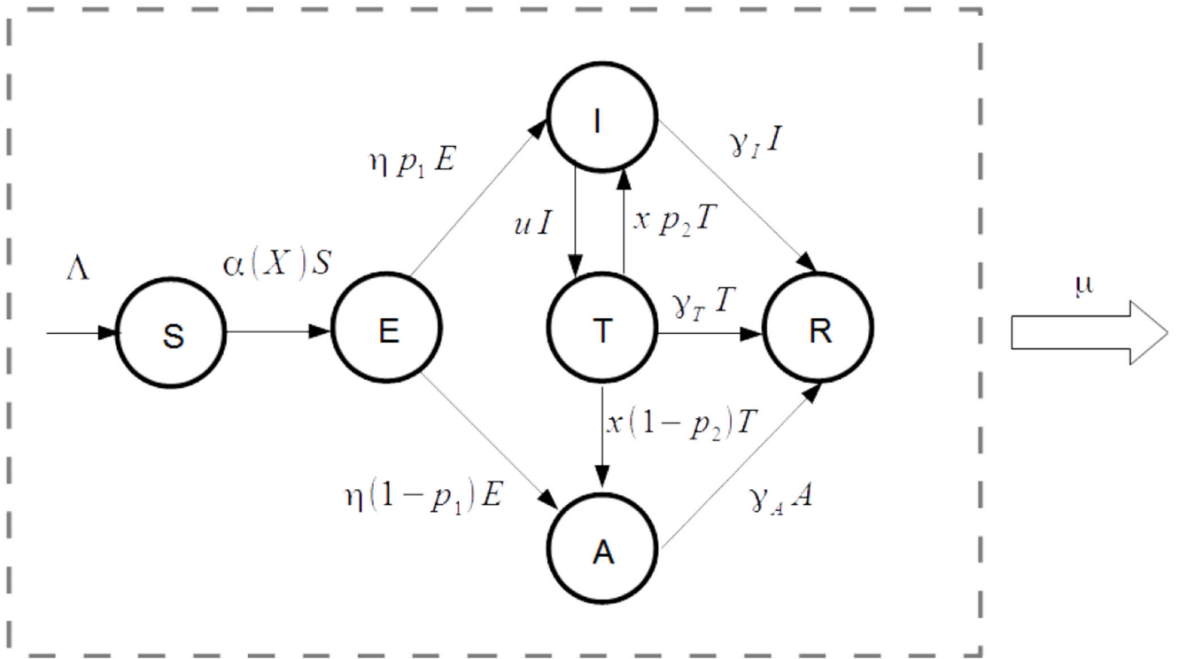
Figure 2: SEIR model.
