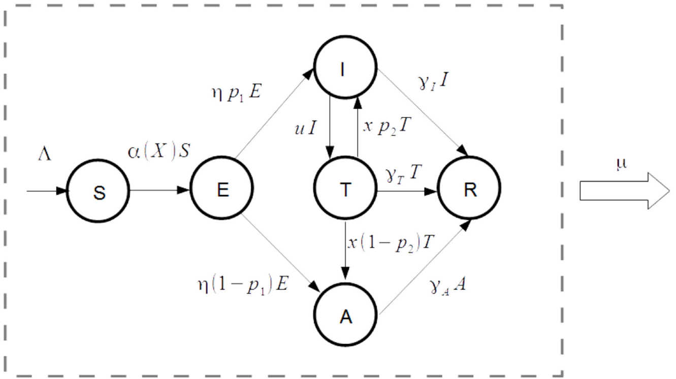
Figure 2: SEIR model.
