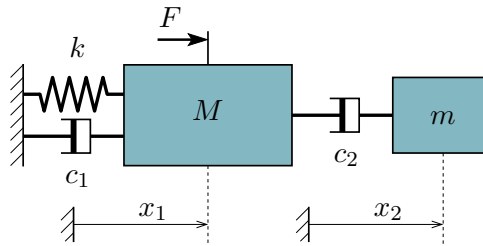
Figure 1: Schematics of a linear Lanchester absorber connected to a primary system of mass M
