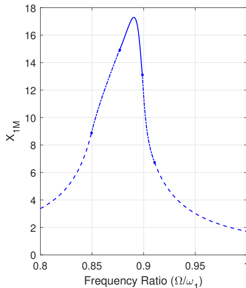
Figure 12: Frequency response for the primary system of figure 9 with \xi = 0.01 , \mu = 0.1 and \lambda = 0.7 . Continuous line shows slip only response, dash-dotted lines shows stick-slip response and dashed lines shows the stick-only response type. circles (o) indicate switching points between response types.
