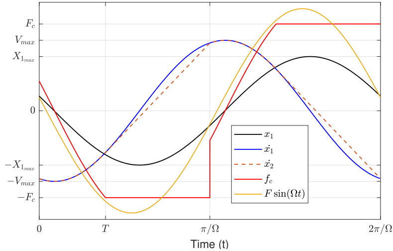
Figure 10: Representation and characteristics of a stick-slip response for the two dof system of fig.9. Arbitrary units for y -axis.
