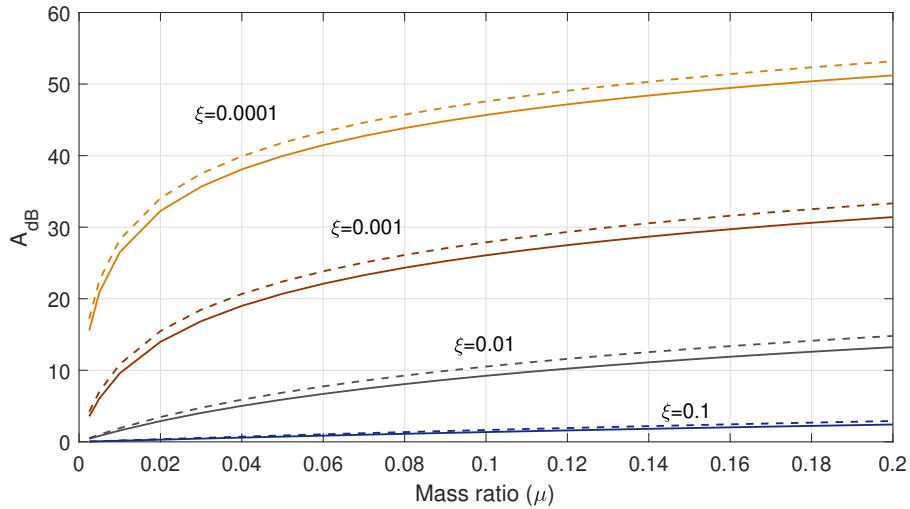
Figure 18: Comparison of the efficiency A_{dB} between linear and non linear dampers, as function of \mu , for different values of \xi . Continuous lines are related to non linear damper and dashed lines are related to the linear damper.
