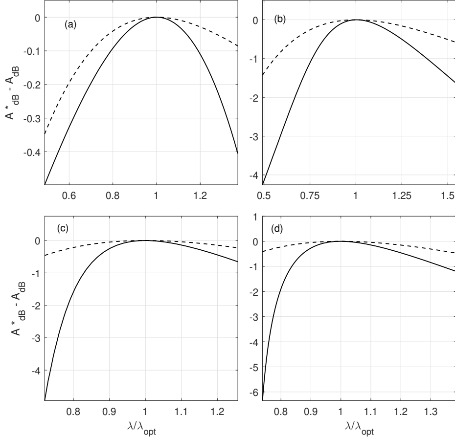
Figure 19: Efficiency drop ( A_{dB}^* - A_{dB} ) for both linear (dashed lines) and non linear (continuous lines) for different values of \xi , with \mu = 0.1 . (a): \xi = 10^{-1} , (b): \xi = 10^{-2} , (c): \xi = 10^{-3} , (d): \xi = 10^{-4}
