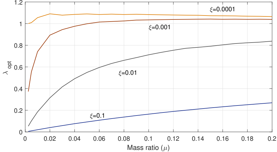
Figure 16: Optimal values of \lambda for the non linear Lanchester damper, as a function of the mass ratio \mu , for several values of \xi .
