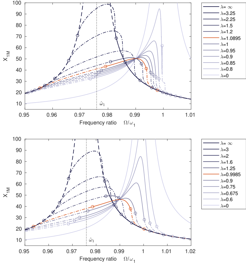
Figure 13: Frequency response of the primary mass for \xi = 10^{-4} (top plot) and \xi = 10^{-3} (bottom plot) with \mu = 0.05 . Continuous line shows slip-only response, dash-dotted lines shows stick-slip response and dashed lines shows the stick-only response type. Circles (o) indicate switching points between response types. The colors are related to a given value of \lambda , shown in the legend.
