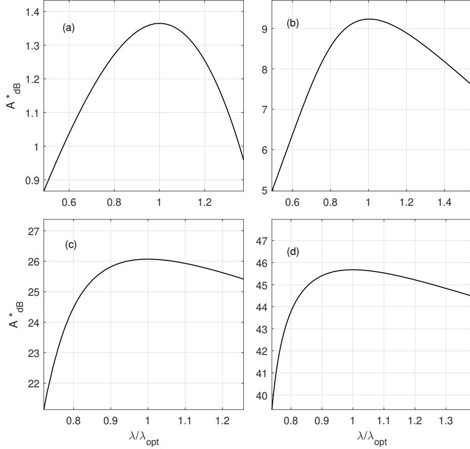
Figure 17: Efficiency ( A^*_{dB} ) as function of deviation of \lambda from its optimal value ( \lambda_{opt} ) for different values of \xi , with \mu = 0.1 . (a): \xi = 10^{-1} , (b): \xi = 10^{-2} , (c): \xi = 10^{-3} , (d): \xi = 10^{-4}
