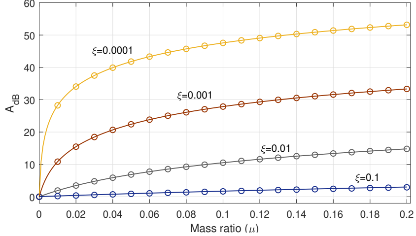
Figure 6: Comparison between numerical and analytical values of A_{dB} as a function of mass ratio ( \mu ) for several values of \xi . Continuous lines (—) relate to the numerical method and circles ( \circ ) relate to the analytical method
