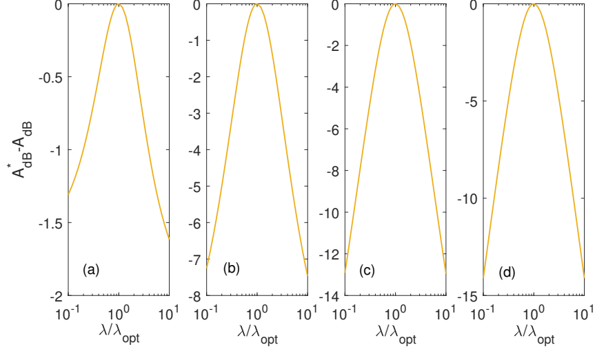
Figure 8: A_{dB}^* - A_{dB} as function of deviation of \lambda_{opt} for several values of \xi and \mu . (a): \xi = 0.1 , (b): \xi = 0.01 , (c): \xi = 10^{-3} and (d) \xi = 10^{-4} .
