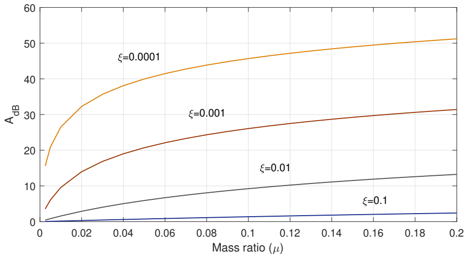
Figure 15: Efficiency A_{dB} of the non linear Lanchester damper, as a function of the mass ratio \mu for several values of \xi .
