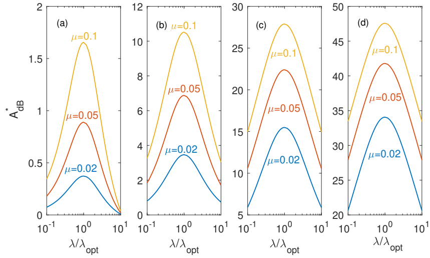
Figure 7: A_{dB}^* as function of deviation of the design parameter from its optimal value ( \lambda/\lambda_{opt} ) for several values of \xi and \mu . (a): \xi = 0.1 , (b): \xi = 0.01 , (c): \xi = 10^{-3} and (d) \xi = 10^{-4} .
