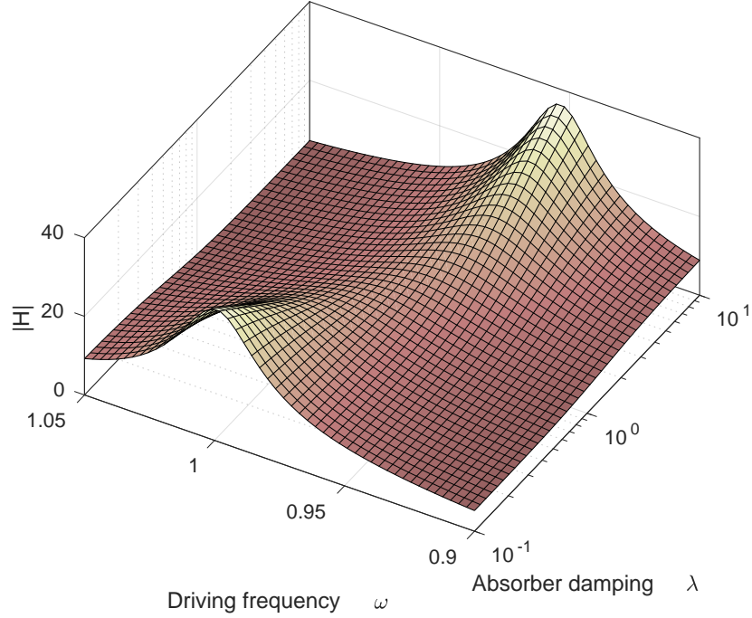
Figure 2: Surface of modulus |H(\omega)| for a primary system with parameters \xi = 0.01 and \mu = 0.1
