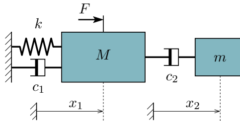
Figure 1: Schematics of a linear Lanchester absorber connected to a primary system of mass M
