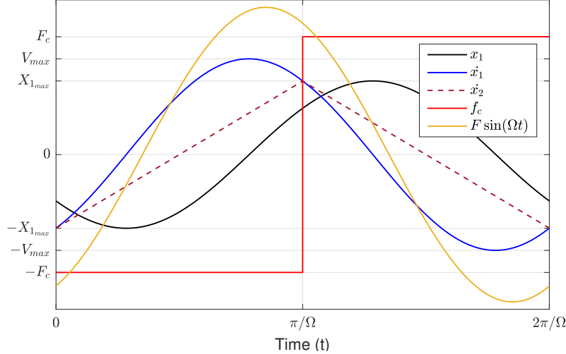
Figure 11: Representation and characteristics of a slip only response for the two dof system of fig.9. Arbitrary units for y -axis.
