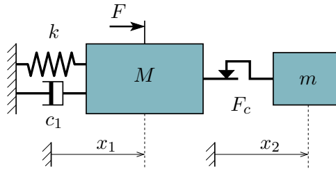
Figure 9: Schematics of a non linear Lanchester absorber attached to a primary system of mass M
