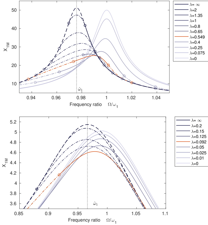
Figure 14: Frequency response of the primary mass for \xi = 0.01 (top plot) and \xi = 10^{-1} (bottom plot) with \mu = 0.05 . Continuous line shows slip-only response, dash-dotted lines shows stick-slip response and dashed lines shows the stick-only response type. circles ( \circ ) indicate switching points between response types. The colors are related to a given value of \lambda , shown in the legend.
