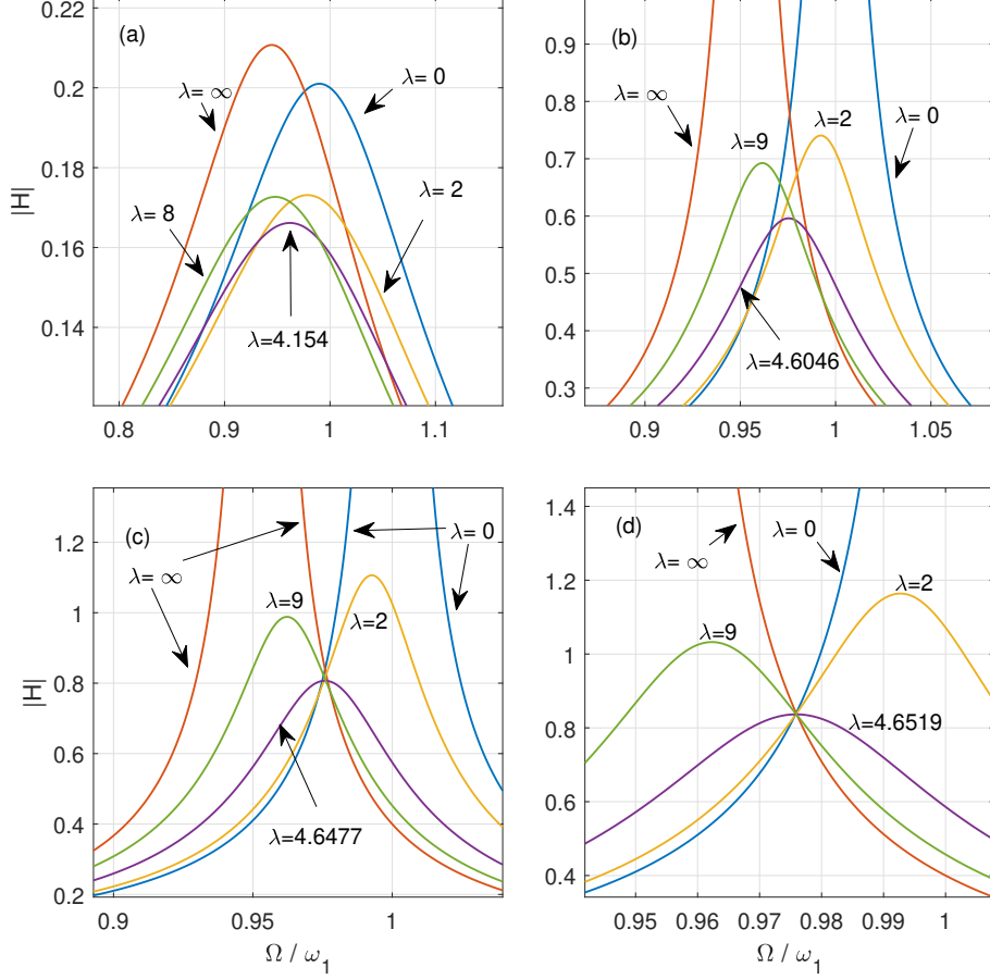
Figure 5: Frequency response function of the primary mass for different values of \xi and \lambda . (a): \xi = 0.1 , (b): \xi = 0.01 , (c): \xi = 10^{-3} and (d) \xi = 10^{-4} .
