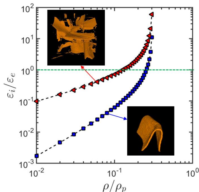
Figure 11. Estimated evolutions of \varepsilon_c/\varepsilon_e (red triangles) and \varepsilon_r/\varepsilon_e (blue squares) with the relative density \rho/\rho_p .
