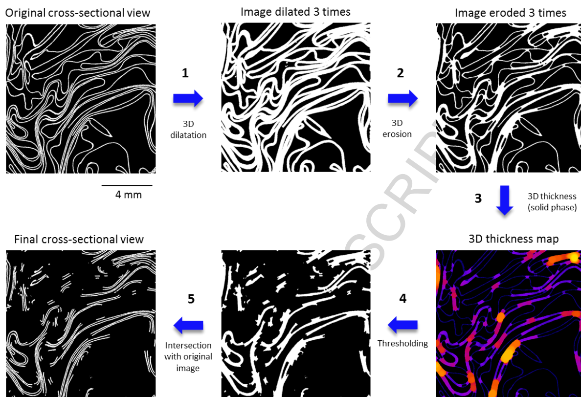
Figure 3. Set of image processing operations applied on binarized stacks to separate the layered domains in crumpled materials.
