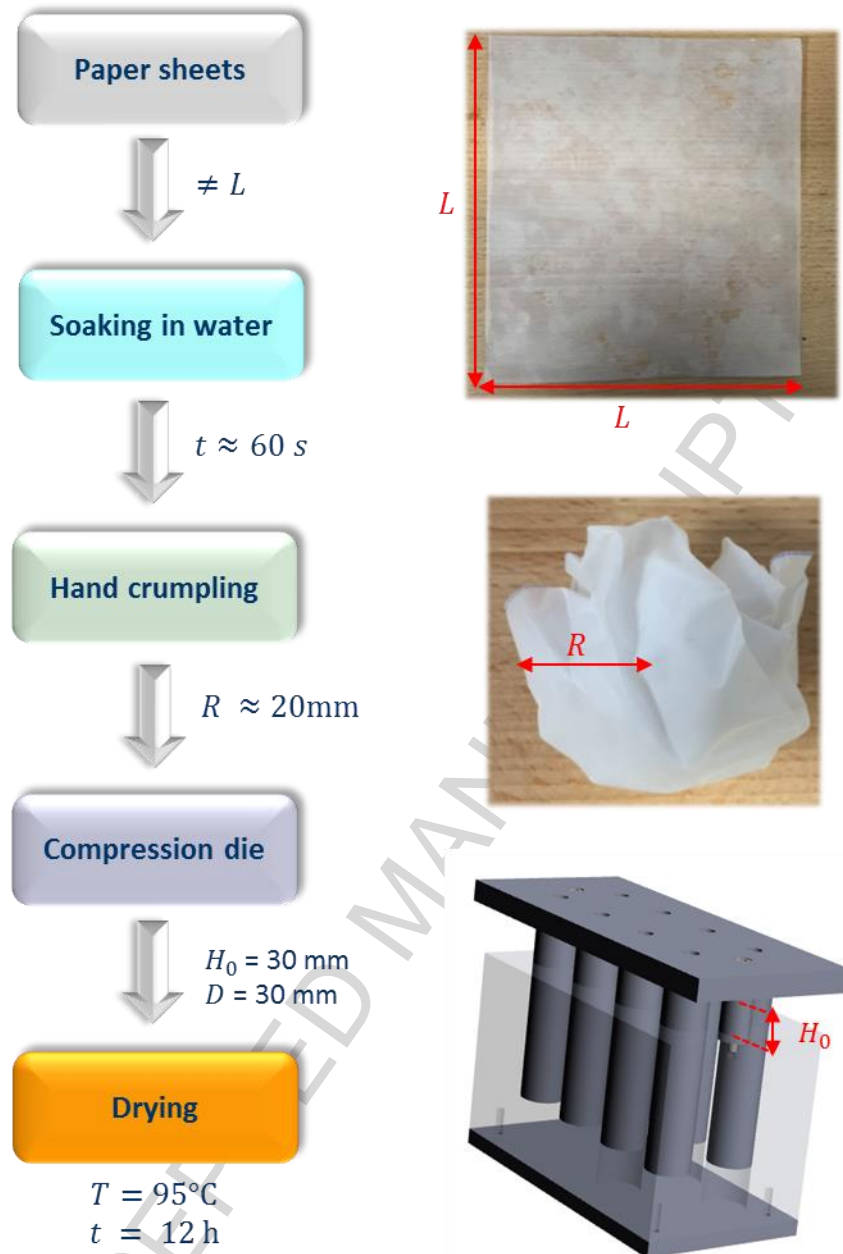
Figure 2. Scheme of the procedure used to fabricate crumpled paper-based materials. The fabricated samples were conditioned in controlled environmental conditions ( T = 25^\circ\text{C} , relative humidity of 50%) for at least two days before testing.
