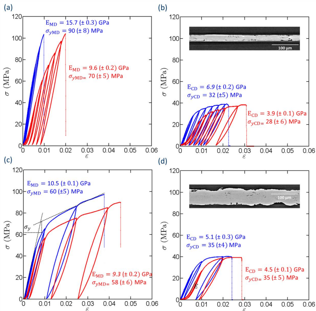
Figure 1. (a,b) Tensile stress \sigma as a function of logarithmic (Hencky) strain \epsilon obtained for tracing (a,b) and crystal paper sheets (c,d) in the machine direction (MD) (a,c) and in the cross direction (CD) (b, d). The blue curves correspond to the mechanical response of initial sheets, whereas the red curves correspond to the mechanical behavior of paper sheets after being soaked in water for 60 s and dried in an oven at a temperature of 95°C. The insets of figures b,d correspond to 2D cross section views of (a) tracing and (b) crystal paper obtained using X-ray synchrotron microtomography (voxel size: 0.6^3 \mu\text{m}^3 ). The Young's moduli and yield stresses reported in these graphs are based on an average of 5 measurements. The first were estimated at the onset of unloading specimen after stretching them up to \epsilon \approx 0.005 , the second were estimated according to the method shown in (c).
