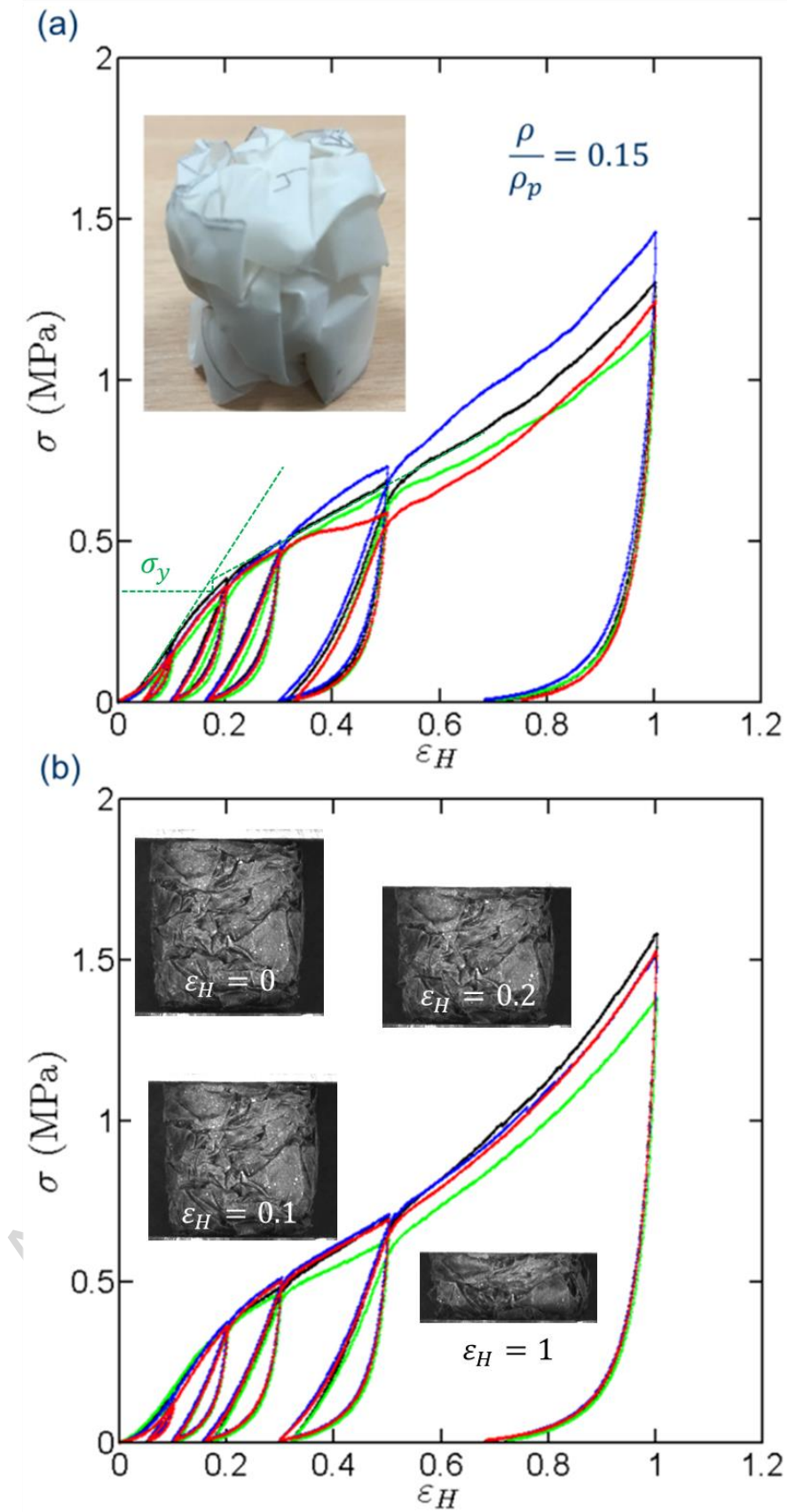
Figure 9. Stress-strain curves of crumpled structures obtained during the compression of tracing (a) and crystal (b) paper sheets with very close relative density. The image insets show the evolution of the geometry of a crumpled crystal sample during simple compression.
