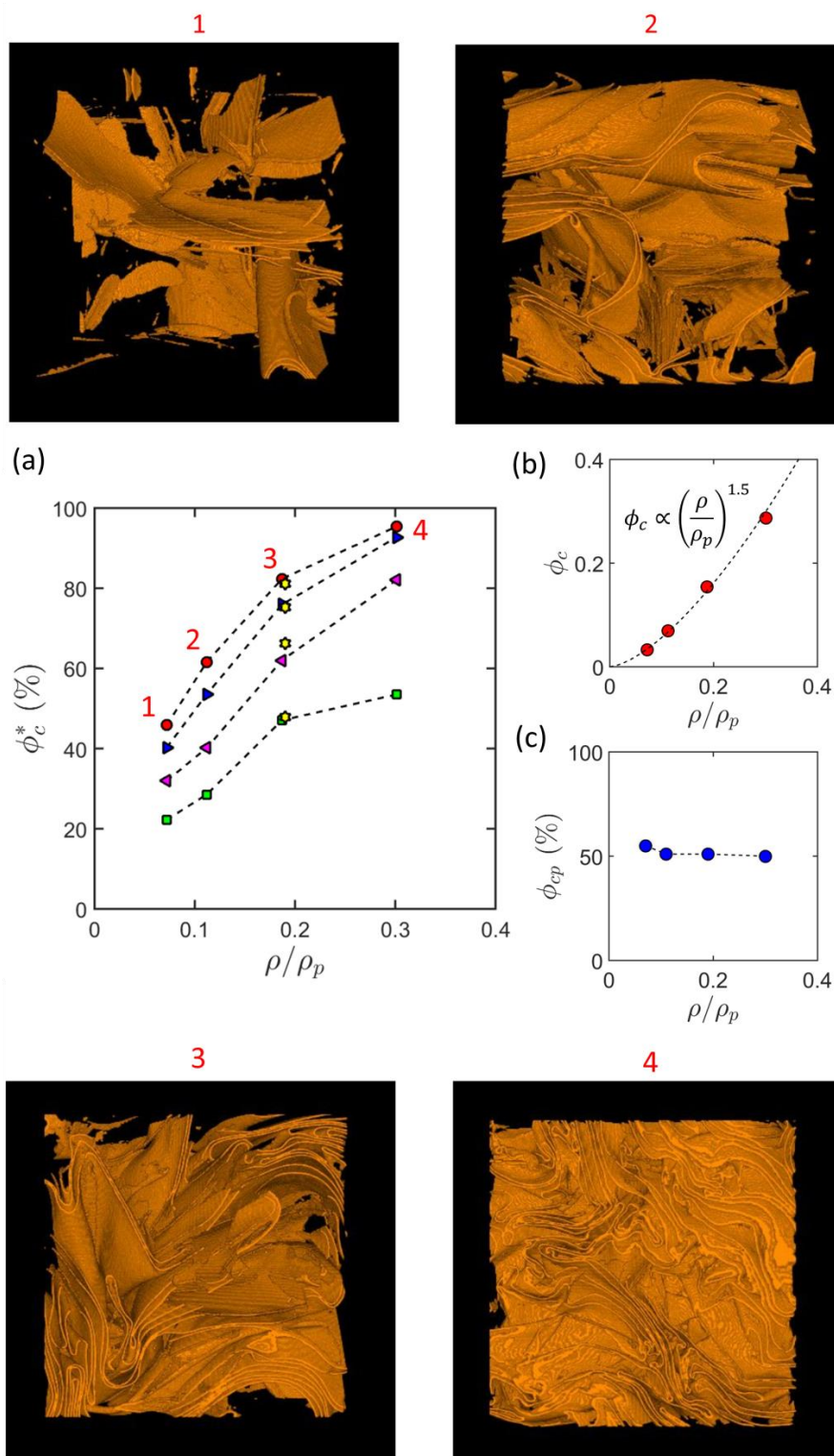
Figure 7. (a) Evolution of the relative volume fraction of layered stacks \phi_c^* = \phi_c/(\rho/\rho_p) as a function of the relative density \rho/\rho_p . The green, magenta, blue and red symbols were obtained for the tracing paper. They correspond to values of \phi_c obtained by keeping only the ordered zones with a thickness t_c between the interlayered sheets of interlayer thickness equal to \bar{t} , 2\bar{t} , 3\bar{t} and 4\bar{t} , respectively. The yellow star symbols were estimated with a crumpled crystal sheet. The 3D views (size of 12 \times 12 \times 12 \text{ mm}^3 ) represent the layered domains in crumpled tracing materials for different relative densities and
