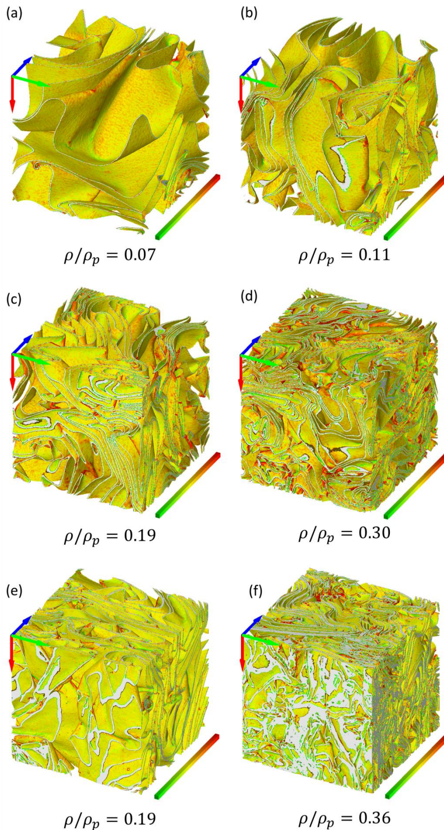
Figure 4. 3D views of crumpled tracing sheets (a-d) and crystal sheets (e-f). The colormaps represent the mean curvature of the sheets (see subsection 2.3) that range from -50 (green, concave shape) to 50 \text{ mm}^{-1} (red, convex shape). For better visualization, curvatures are represented on all interface
