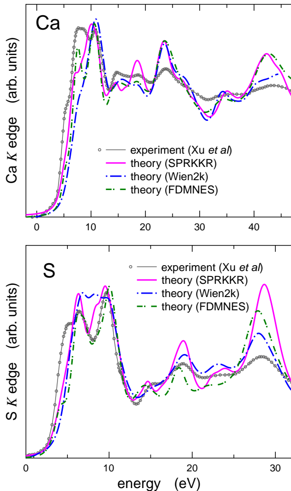
FIG. 1. Experimental Ca K edge (upper panel) and S K edge (lower panel) XANES of CaS [8] together with theoretical spectra obtained using the full-potential multiple-scattering method (SPRKKR code), the FLAPW method (WIEN2K code), and the full-potential FDM (FDMNES code).
