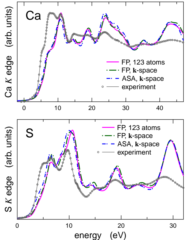
FIG. 2. Theoretical Ca K edge (upper panel) and S K edge (lower panel) XANES of CaS obtained in the full-potential (FP) mode either in the real space (for a cluster of 123 atoms) or in the reciprocal space, together with XANES obtained for a spherical potential (ASA) in the reciprocal space. The calculations were done using the SPRKKR code, the core hole was not taken into account. Experimental XANES of Xu et al. [8] is shown for comparison.
