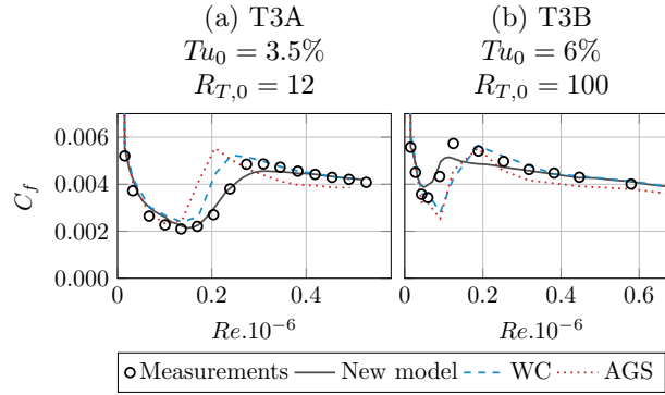
Figure 8: Skin friction coefficient for the ERCOFTAC T3A (a) and T3B (b) cases (symbols), calculated with the new model (plain line), the Walters & Cokljat model (WC, dashed line) and the Abu-Ghannam and Shaw criterion (AGS, dotted line).
