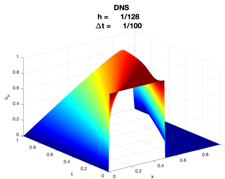
Figure 1. DNS solution obtained by using a piecewise linear finite element spatial discretization and the backward Euler time discretization.
