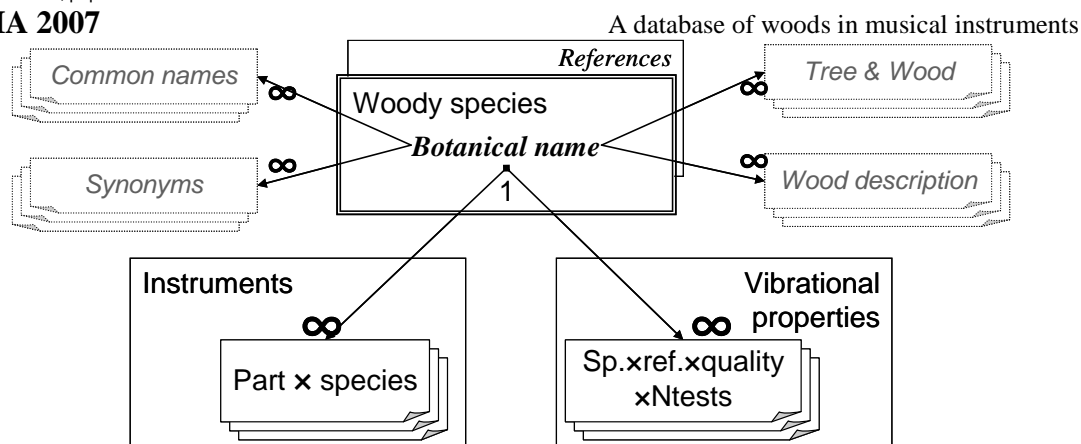
Figure 1: Schematized structure of the database and its relations. (Links to wood properties are also possible with any other existing database with records defined by “botanical name”)
