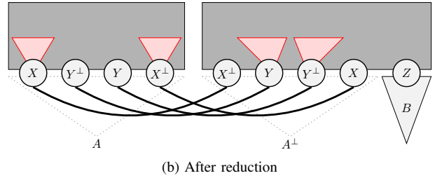
Fig. 4: Public reduction
