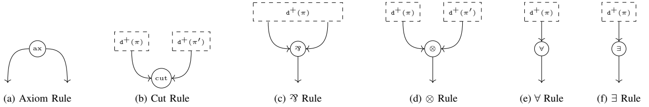
Fig. 1: Translation d^+(\_) .
