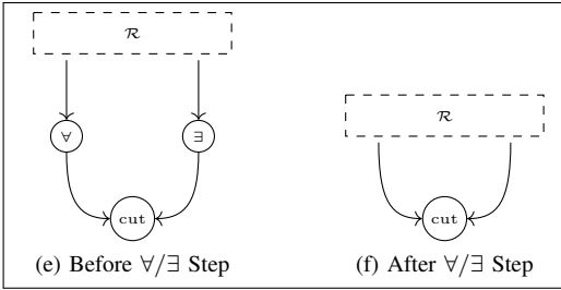
Fig. 2: Cut Elimination Steps.
