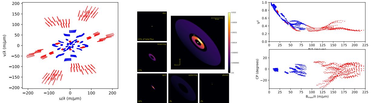
Figure 1. Leftmost panel: u,v coverage of the data set. CHARA/MIRC data points are in red, whereas VLTI/PIONIER data points are in blue. Central panels: Model used to generate the synthetic data showing each component described in the text, as well as a synthetic image (large upper right panel) in non linear colour scale. Rightmost panels: V^2 (upper) and phase closure (lower) as a function of spatial frequency. Same colour code as the leftmost panel.
