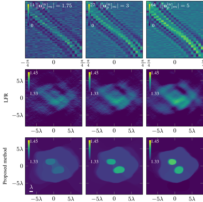
Fig. 3. Noisy measurements and their RI reconstructions. Each column corresponds to a noise level. From left to right: ||\mathbf{u}_p^{\text{in}}||_m = 1.75 , ||\mathbf{u}_p^{\text{in}}||_m = 3 , ||\mathbf{u}_p^{\text{in}}||_m = 5 \forall p \in [1 \dots P] . Top to bottom: intensity measurements, LFR [20], and proposed method.
