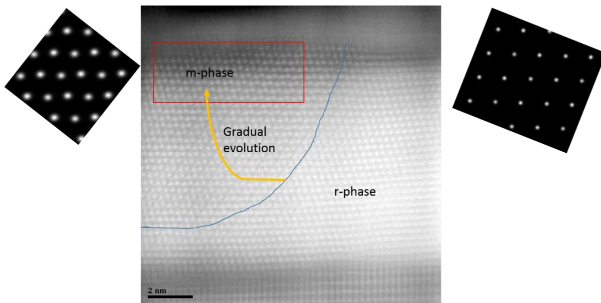
Figure S4: Evolution to a monoclinic (bulk) phase with thickness. HAADF-STEM cross-section image ( ZA , \varphi=45^\circ ) of a 9 nm HZO sample showing a gradual evolution of r-phase into bulk-m phase with increasing thickness. (inset left), HAADF-STEM simulation of an m-phase clearly showing the zig-zag atomic positions along [112] (horizontal direction), (right) Corresponding HAADF-STEM image simulation. Renditions of various rhombohedral structures obtained from our structural search are shown in Fig. S6.
