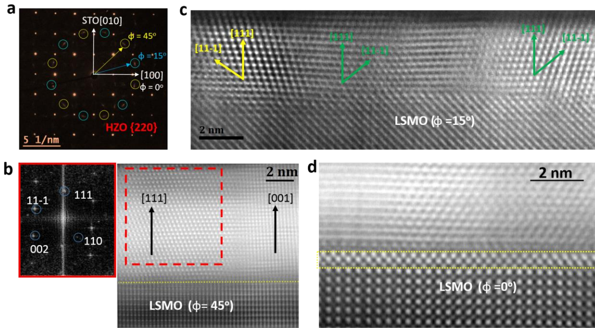
Figure 3: Electron microscopy characterization. a , Plane view selected area electron diffraction (SAED) pattern from a 9 nm thick HZO sample. The out of plane direction is [111] (zone-axis). The \{220\} spots ( d_{220}=1.79 \text{ \AA} ), corresponding to at least two different domains (yellow and blue circles, respectively) rotated by 90^\circ with respect to each other, can be clearly identified. b , Cross-sectional (x) HAADF-STEM image (corrected by sample drift) of the 9 nm thick HZO film, observed along the [110] zone of the substrate ( \phi = 45^\circ ); (inset, left) Fourier transform of the [111] domain; c , Representative x-HAADF STEM image (drift-corrected) of a 4 nm thick film, observed along the zone axis defined by \phi = 15^\circ . (d) HAADF-STEM image observed along STO [100] , revealing a clear interfacial t-phase of HZO (see EDX in Supplementary Fig. S3).
