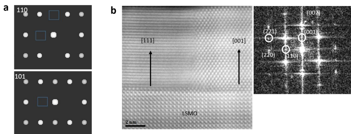
Figure S1. SAED simulations of the polar orthorhombic phase ( Pca2_1 ). a , SAED diffraction simulations of Pca2_1 phase, along the [110] and [101] zone axes. Along the [110] zone, we note that both the (001) and the (1-10) spots are forbidden. Along the [101] zone, (10-1) is forbidden, and along [011] (not shown), the (100) spots are forbidden. b , x-HAADF-STEM image from a 9 nm thick sample in the with zone axis: [100]_{\text{STO}} . Domain coexistence (majority c -axis= [111] , and minority c -axis= [001] ) can be clearly observed. Inset on the right shows FFT in which some spots from the 001 domain are indexed and circled. In an orthorhombic Pca2_1 phase, one of the (001) or the (110) spots should be forbidden (by symmetry). However, we see both of them, clearly suggesting that we have a different ferroelectric phase than the commonly reported Pca2_1 phase.
