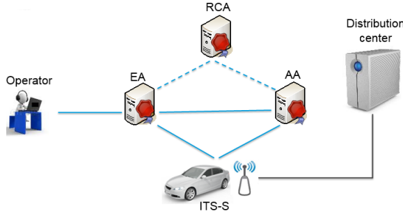
Fig. 1. PKI architecture
