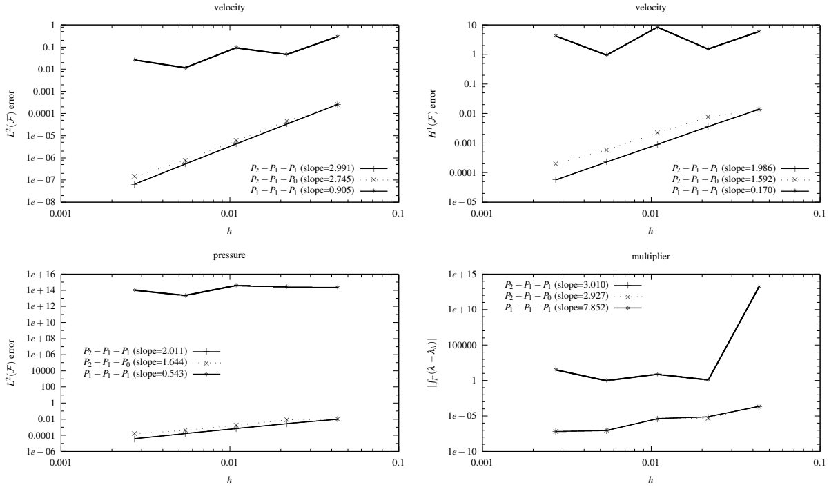
Fig. 4: Rates of convergence without stabilization for \|u - u_h\|_{0,\mathcal{F}} , \|u - u_h\|_{1,\mathcal{F}} , \|p - p_h\|_{0,\mathcal{F}} and |\int_{\mathcal{F}}(\lambda - \lambda_h)|
