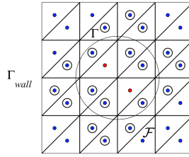
Fig. 2: The meshes \mathcal{T}_h^e = \mathcal{T}_h^i \cup \mathcal{T}_h^\Gamma : the triangles of \mathcal{T}_h^i are marked by • and those of \mathcal{T}_h^\Gamma are marked by ⊙; triangles marked by • are not used.
