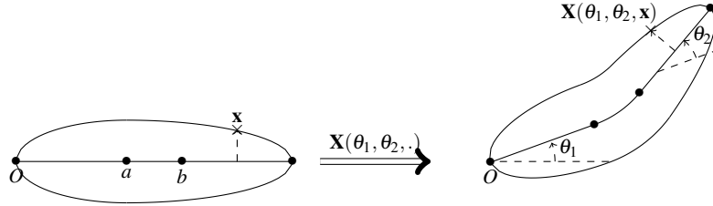
Fig. 7 The diffeomorphism \mathbf{X} .
