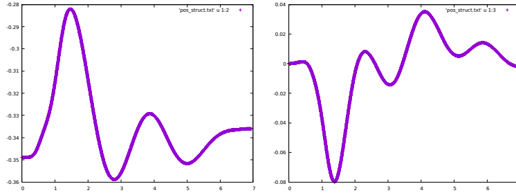
Fig. 9 The evolution of the structure parameters; left: \theta_1 , right: \theta_2 .
