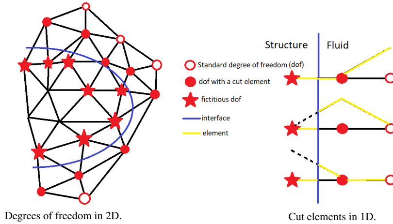
Fig. 2 The degrees of freedom for \mathbb{P}_1 finite elements.
