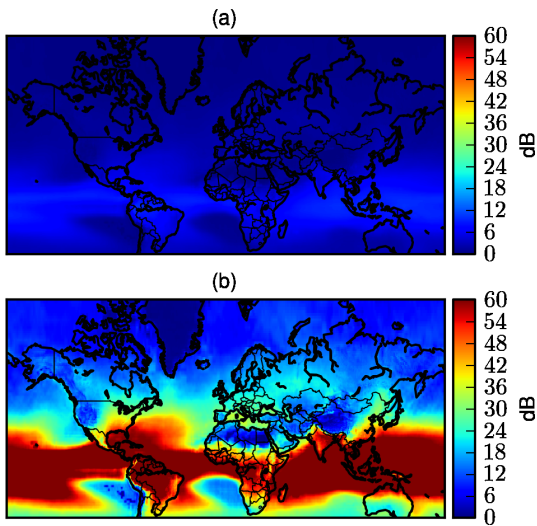
Figure 1. Attenuation that exceeded 0.1 % of the time computed from ITU-R P.618-13 (2017) for a link with a geostationary satellite at 35° of elevation at 12 GHz (a) and 50 GHz (b).
