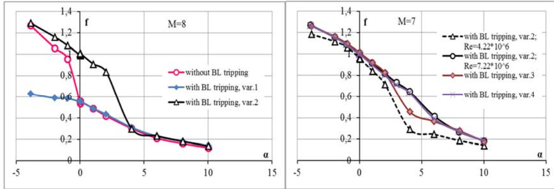
Fig. 38: The intake mass flow rate coefficient f vs. angle-of-attack \alpha . Mach Numbers M_{\infty} = 8 and 7 .
